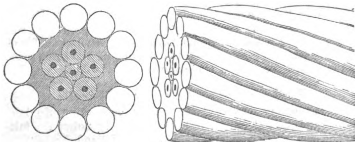
Fig. 8.—Dover and Ostend Cable.
