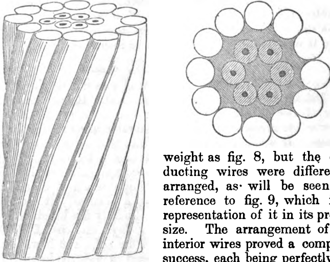
Fig. 9.—Donaghadee and Port Patrick Cable.
