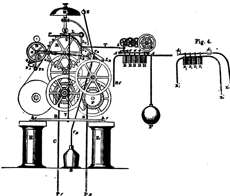
THE PRINTING APPARATUS AND MANIPULATION.
