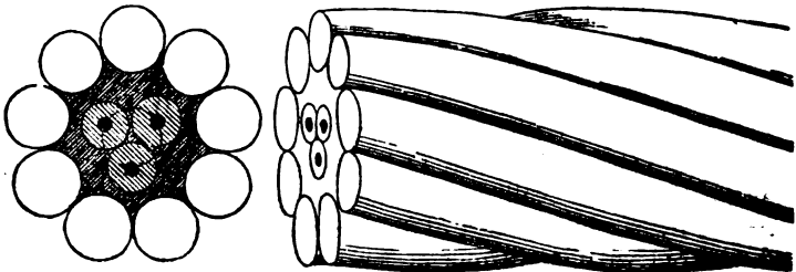
Fig. 12.—Great Belt Cable.
