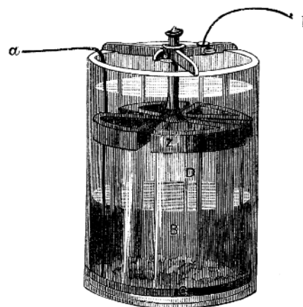
FIG. 5.—THE CALLAUD BATTERY.
