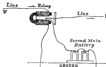
FIG. 16.—PRINCIPLE OF THE REPEATER.
