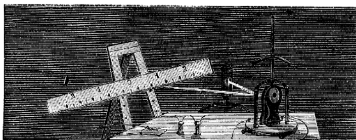
FIG. 27.—THE MIRROR GALVANOMETER.
