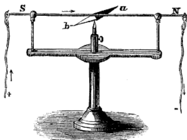
FIG. 7.—THE DEFLECTION OF THE NEEDLE.
