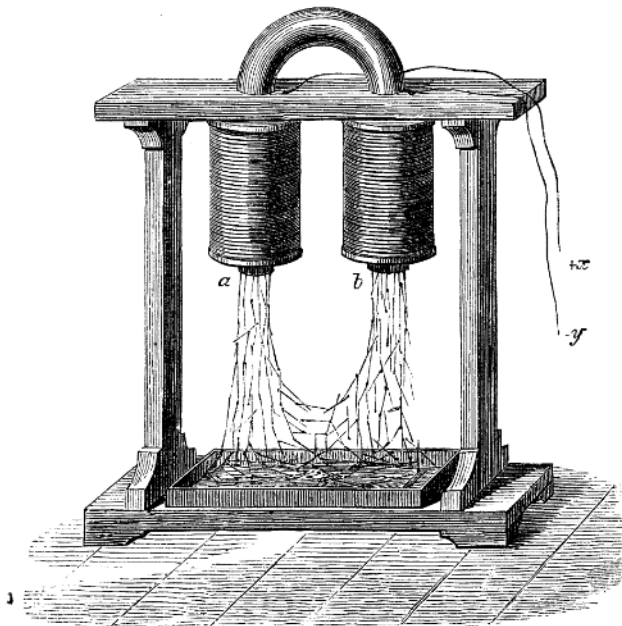
FIG. 10.—THE ELECTRO-MAGNET.
