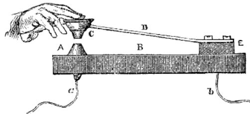
FIG. 14.—THE PRINCIPLE OF THE MORSE KEY.
