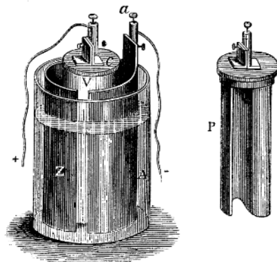
FIG. 4.—A CELL, OR PAIR, IN GROVE'S BATTERY.
