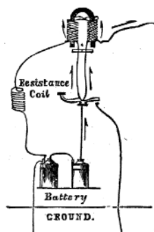
FIG. 26.—PRINCIPLE OF THE DOUBLE TRANSMITTER.
