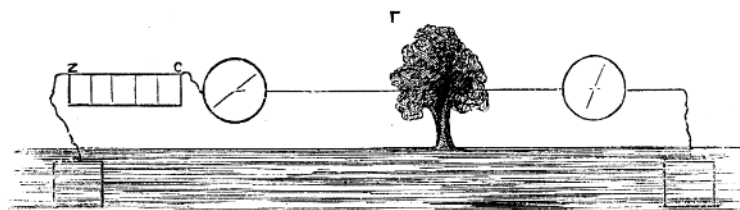
FIG. 20.—PARTIAL EARTH.
