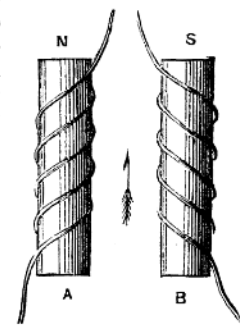
FIG. 9.—THE SPIRALS.
