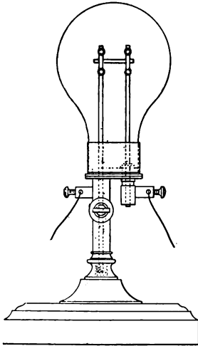
ROBERTS' LAMP, 1852 This consisted of a graphite rod operating in vacuum.
