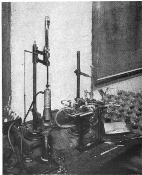
TUBULATING MACHINE, 1903
