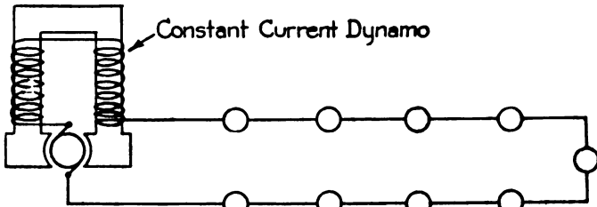
DIAGRAM OF CONSTANT CURRENT SYSTEM
