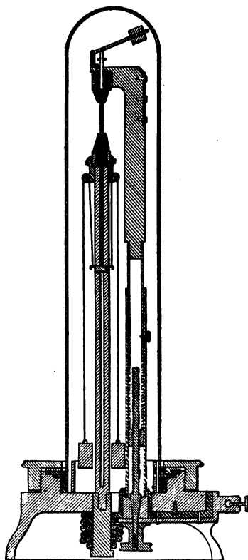
BOULIGUINE'S LAMP, 1876
