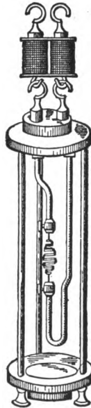
DE CHANGY'S LAMP, 1856 This had a platinum burner operating in air but covered by a glass tube. It was designed for use in a mine, being so arranged that it could be hooked to wires fastened on the walls throughout the mine and thus be located in the places desired.
