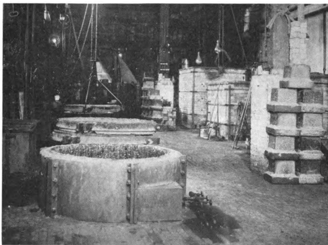
CARBONIZING FURNACES
