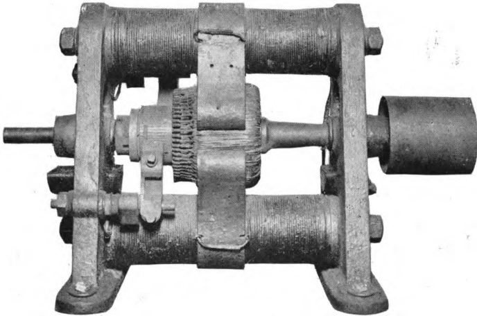
GRAMME'S DYNAMO, 1871
