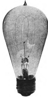
GEM LAMP, 1909 In 1909 it became possible to make a single oval filament for 110-volt service. GEM lamps disappeared from the market in 1918.
