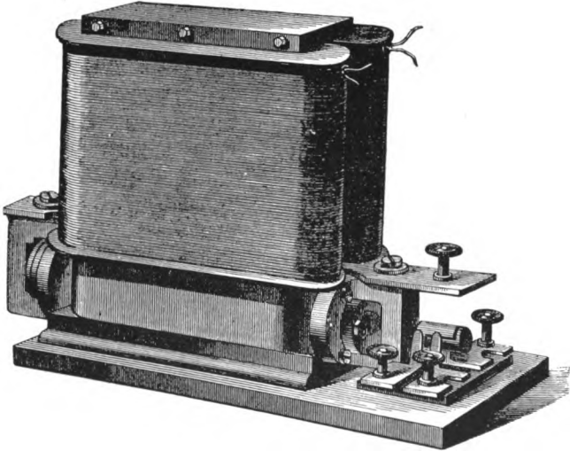
WHEATSTONE'S DYNAMO, 1866
