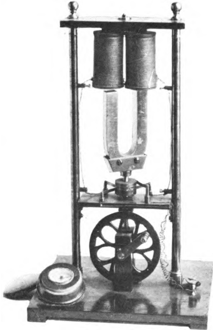
PIXII'S DYNAMO, 1832
