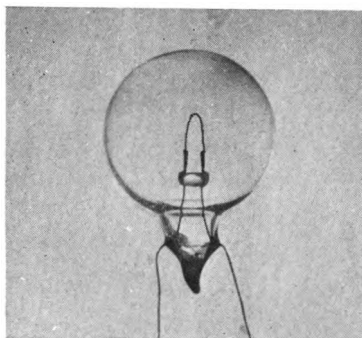
STEMLESS BUTT SEAL
