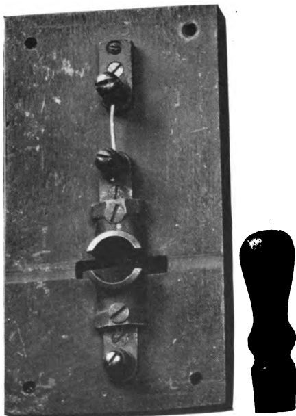
LEAD WIRE FUSE, 1880
