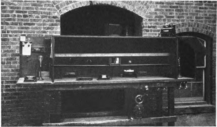
STANDARD PHOTOMETER
