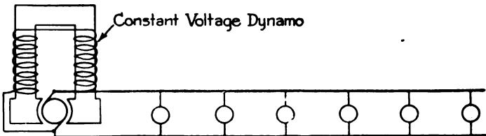
DIAGRAM OF EDISON'S MULTIPLE SYSTEM
