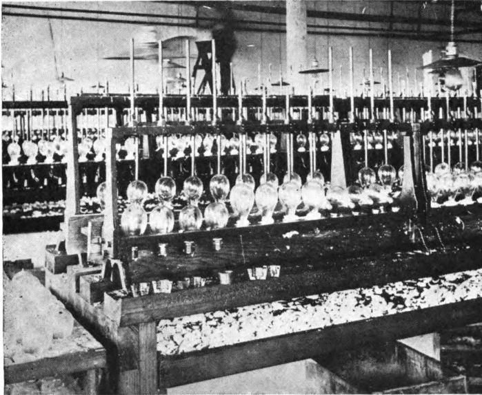
BASING RACK
