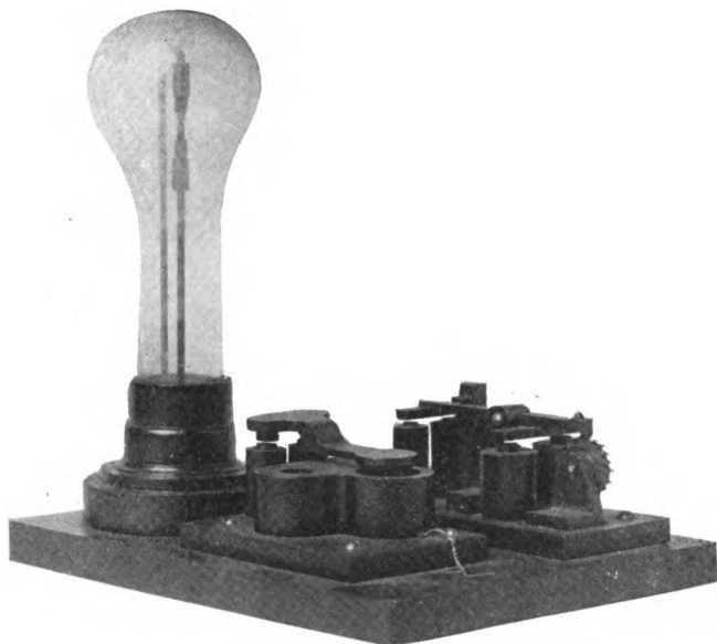
MAXIM'S GRAPHITE LAMP, 1878.
