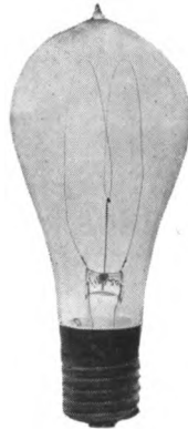
TREATED SQUIRTED CELLULOSE CARBON LAMP, 1894 The lower specific resistance of this filament required that its length be increased, the filament having a loop which was anchored to the stem.
