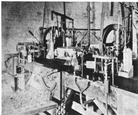
MALIGNANI CHEMICAL EXHAUST, 1896
