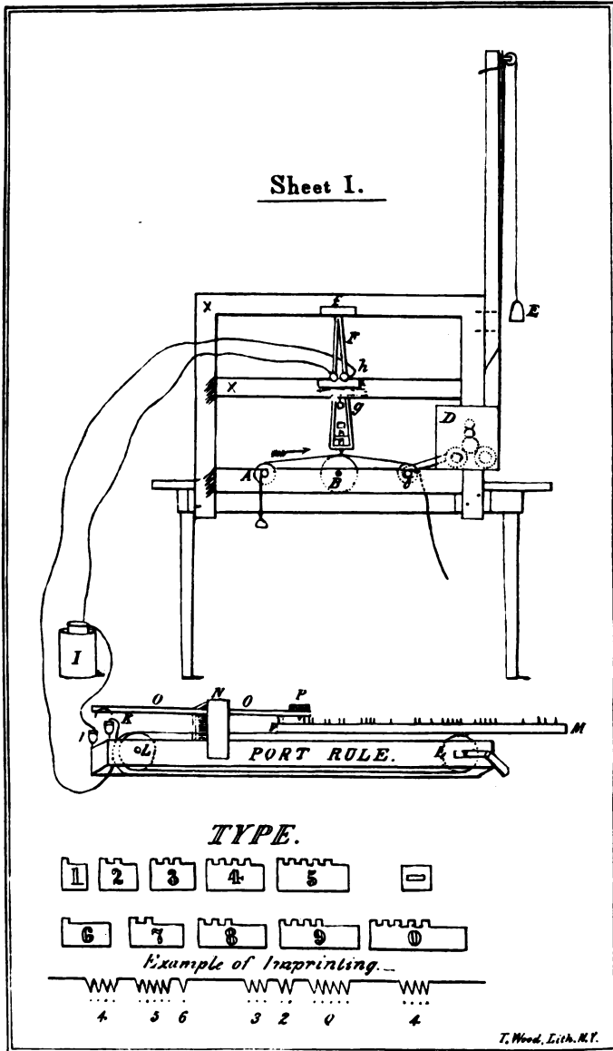
MORSE'S TELEGRAPH OF SEPT. 3, 1837
