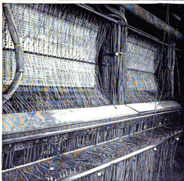
Underside of the Switchboard for 2,000 Wires; Western Union Building, New York.—[Before the Fire.]
