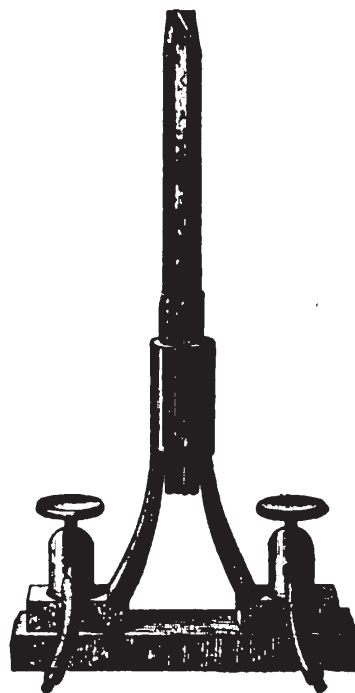
Fig. 11.—The Jablochkoff Candle.
