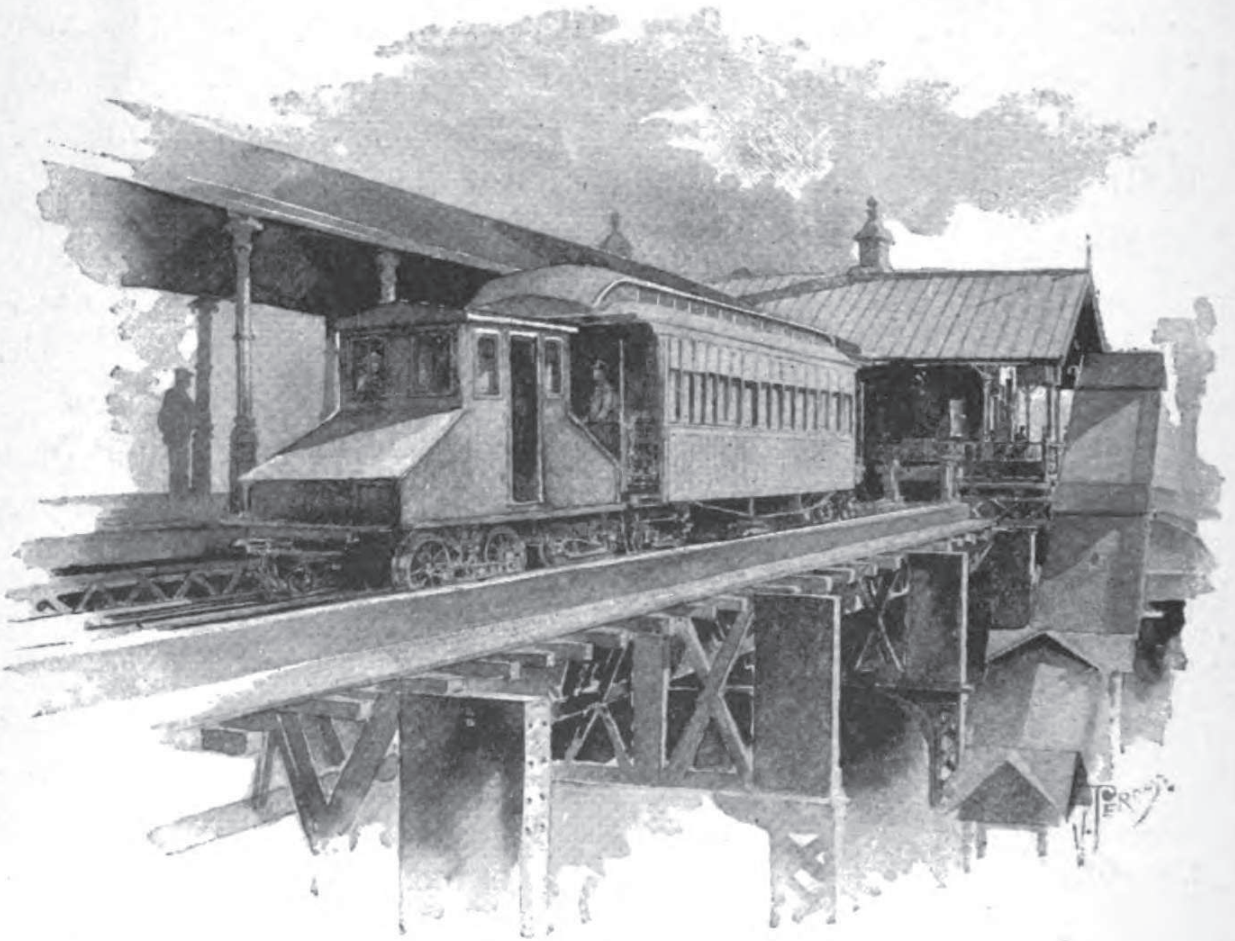
Fig. 11.—Stephen D. Field's Motor.—Experimental Trials on the Thirty-fourth Street Branch of the Elevated Railway, New York City.
