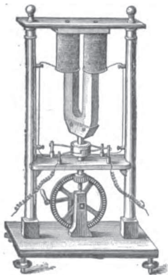
Fig. 1.—Pixii's Magneto-electric Machine, 1832.
