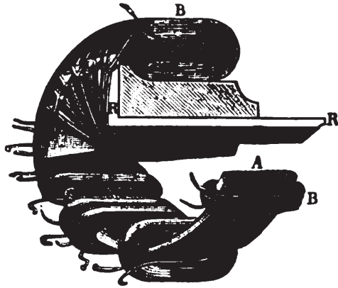
Fig. 5.—Section of a Gramme Armature Ring, showing its construction.
