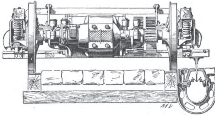
Fig. 8.—The Bentley-Knight Underground Conduit System, showing Cross-section of Track, Conduit, and Truck.
