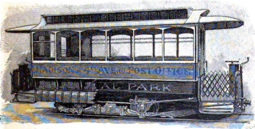
Fig. 9.—The Storage-battery System.—Car of the Julien Electric Traction Company, as run on the Fourth Avenue Road, New York.
