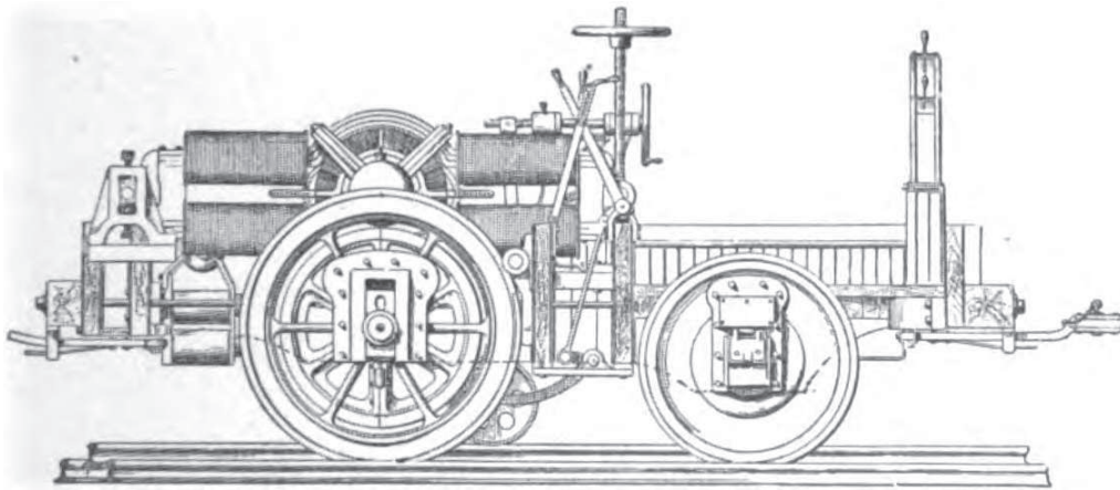
Fig. 10.—Daft Electric Locomotive for Traffic on Elevated Railroads.
