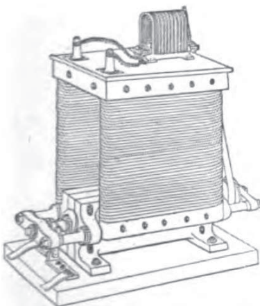
Fig. 4.—The Wilde Machine.
