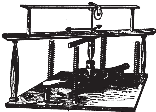
Sturgeon's Electro-magnetic Engine.
