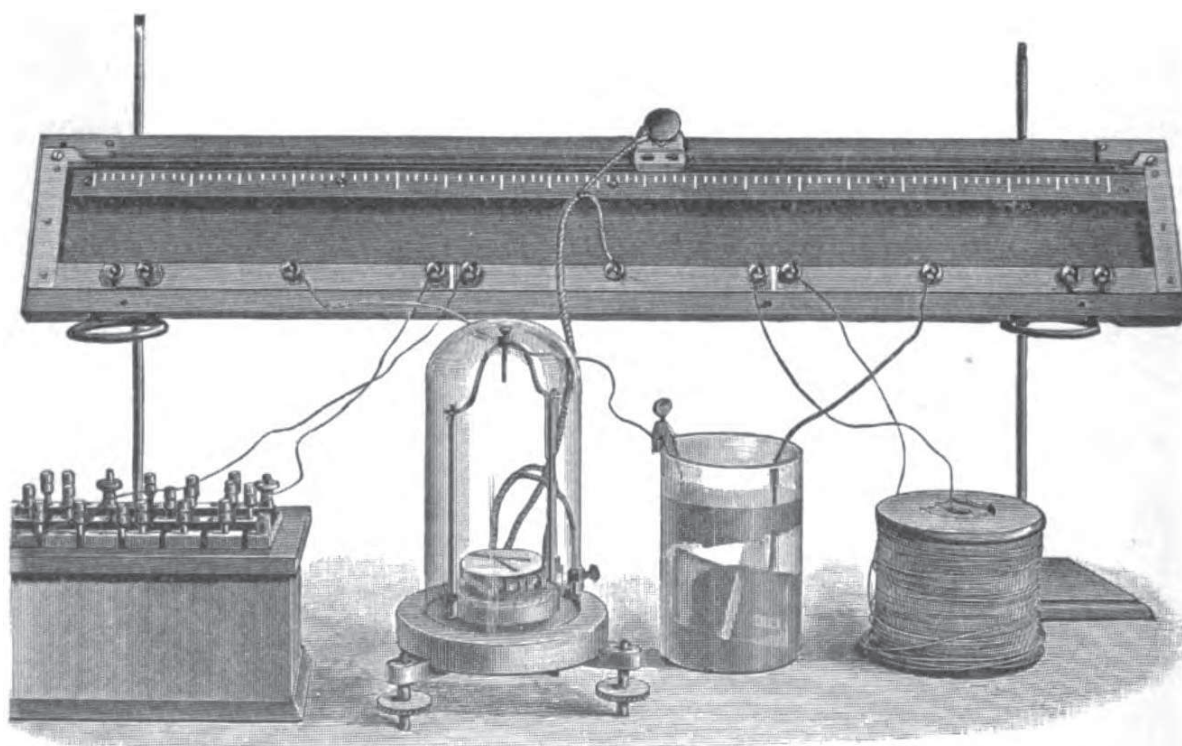
Box of standard resistances. Galvanoscope. Battery. Conductor to be measured. Above, sliding key for effecting balance. Wheatstone's Balance, used for comparing resistances.
