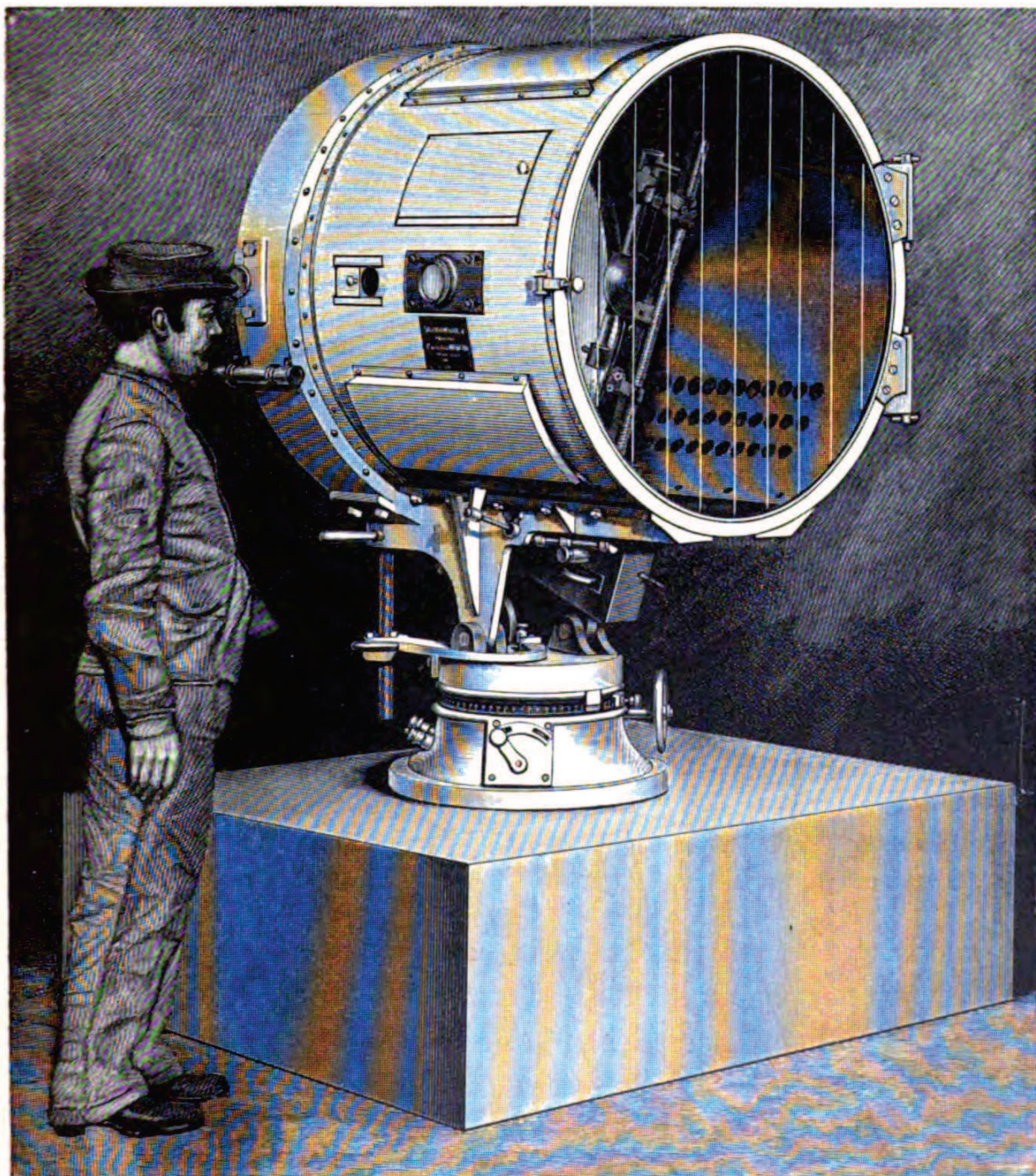
Ship-of-war's Search-light, 25,000 Candle-power.
