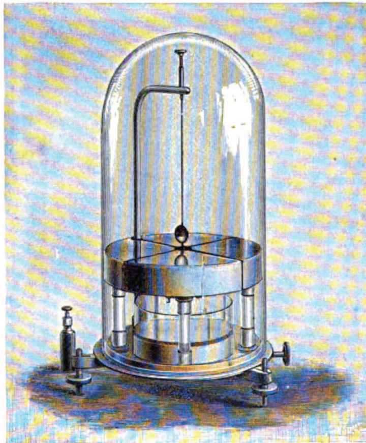
Thomson's Quadrant Electrometer, for comparing potentials.
