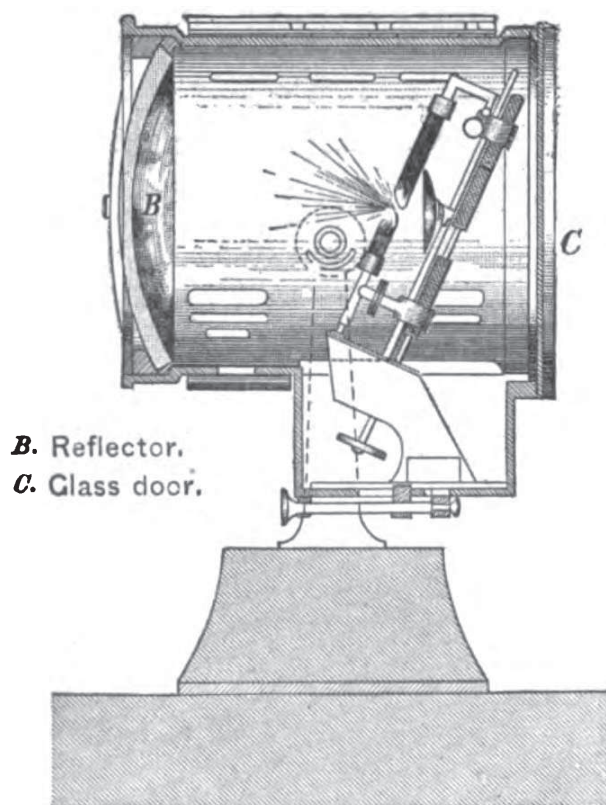
Sectional View of Ship's Search-light.
