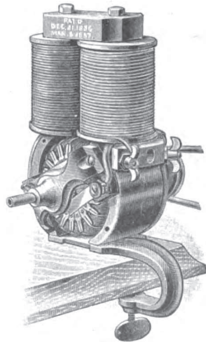
Motor attached to a Sewing-machine.
