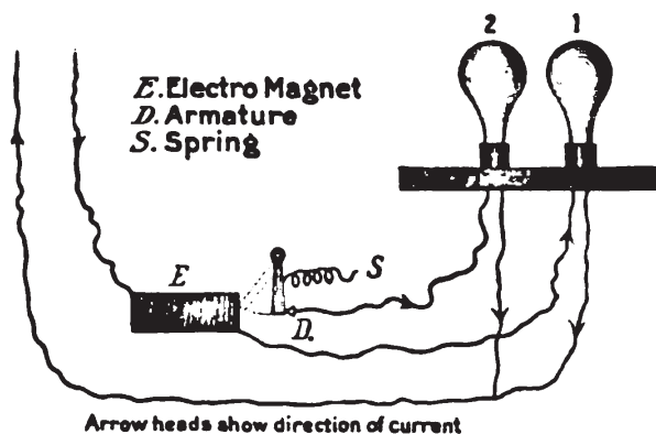
Arrow heads show direction of current Arrangement of Electrical "Running Lights" for Ships.
