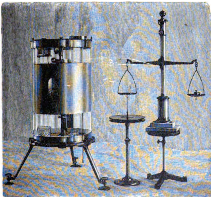
Sir William Thomson's. After the plan of Harris. Electrometers for Measuring Difference of Potential.
