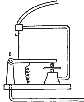
Fig. 15.—Edison's First Incandescent Platinum Lamp.
