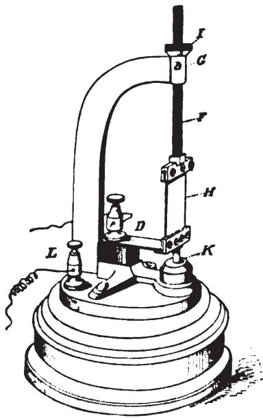
Fig. 17.—Maxim's Incandescent Platinum Lamp.
