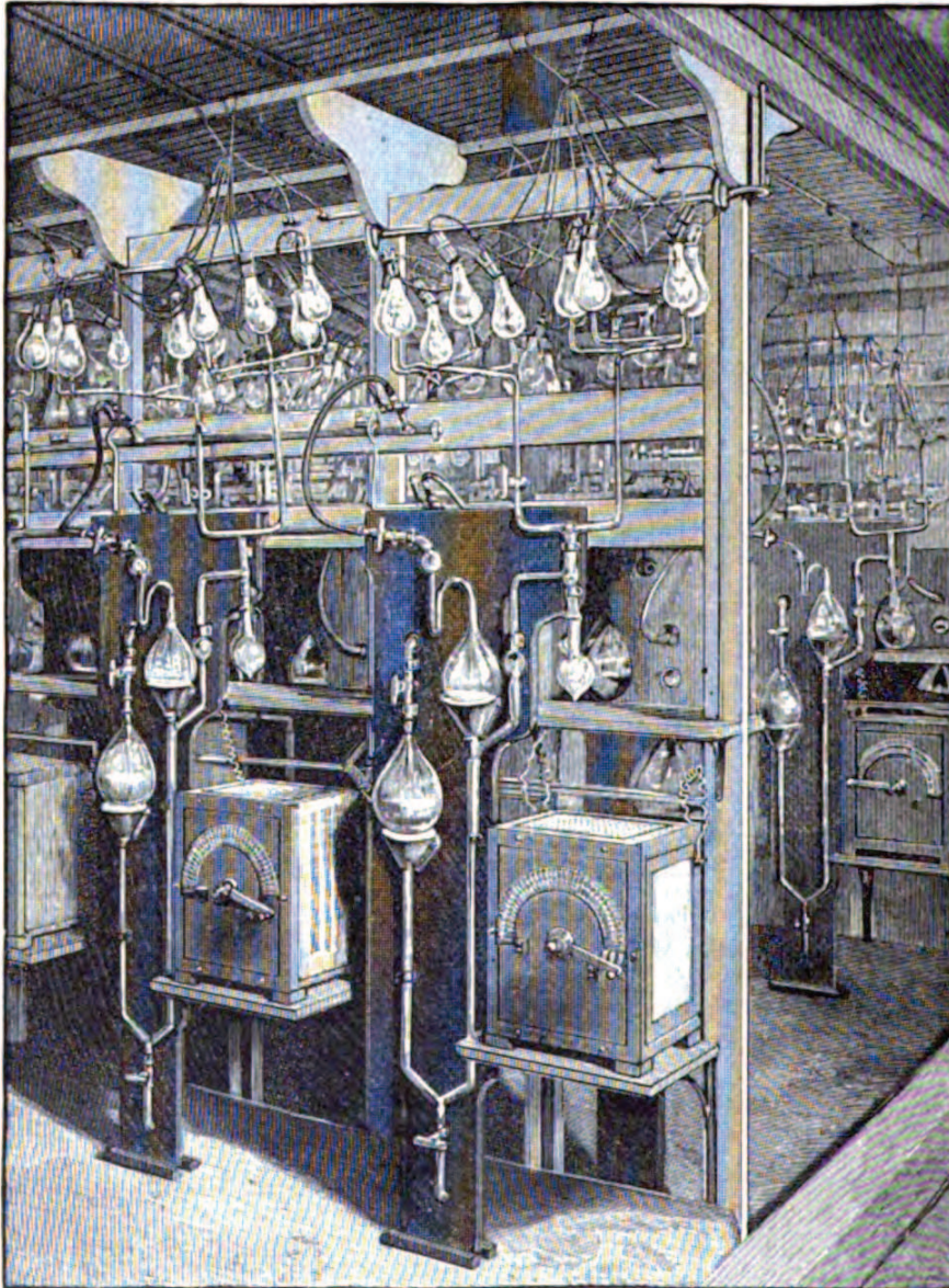
Fig. 21.—The Process of Exhausting the Air from Incandescent Lamps.
