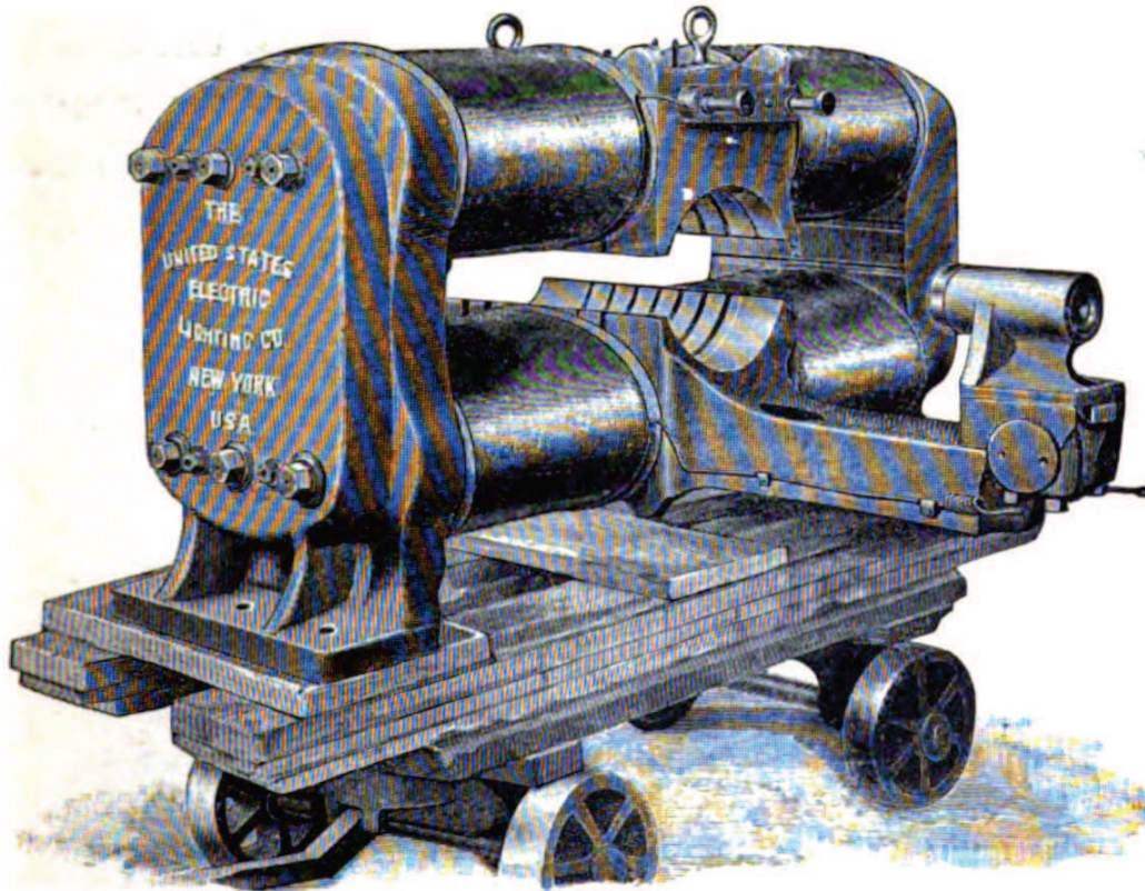
Fig. 9.—Field Magnets and Frame, without armature.
