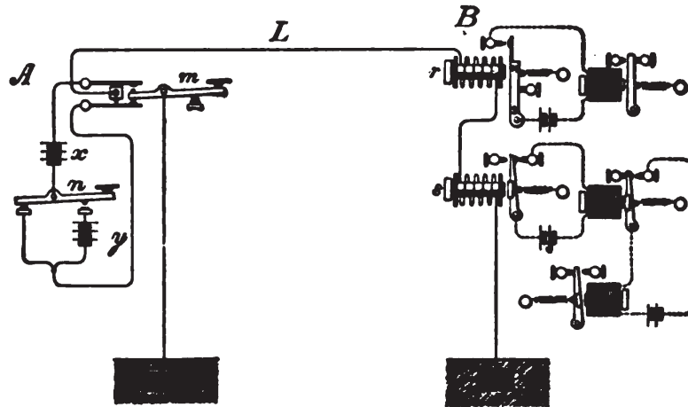
The Diplex System, for simultaneously sending two messages in the same direction on a single wire.
