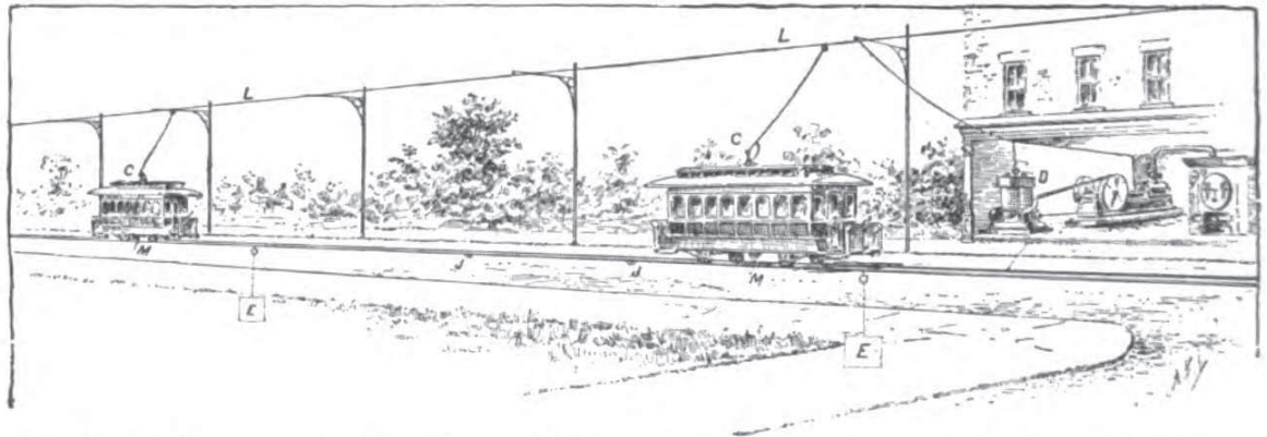
Fig. 2.—Plan showing Principles of Operating the Overhead System of Electric Railways.
