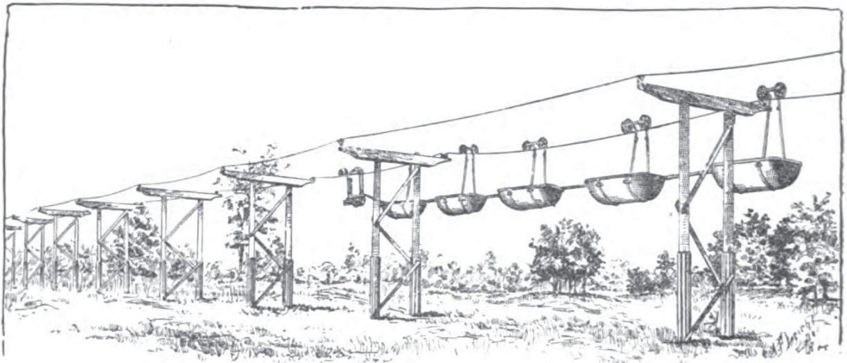
Fig. 12.—The Glynde, England, Telpherage Line, on the System of the Late Fleeming Jenkin.
