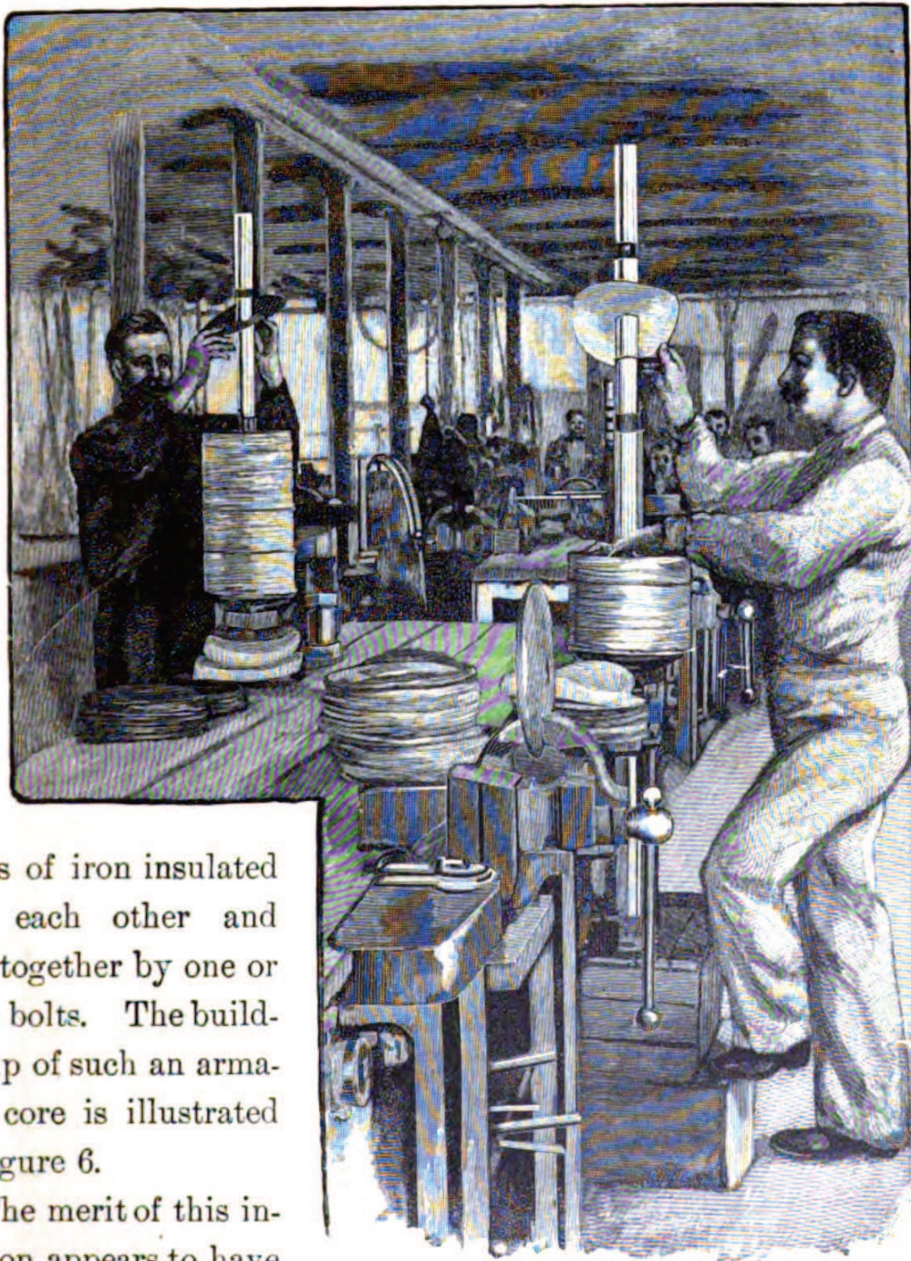
Fig. 6.—Workmen Building up the Armature Core of a Modern Dynamo.
