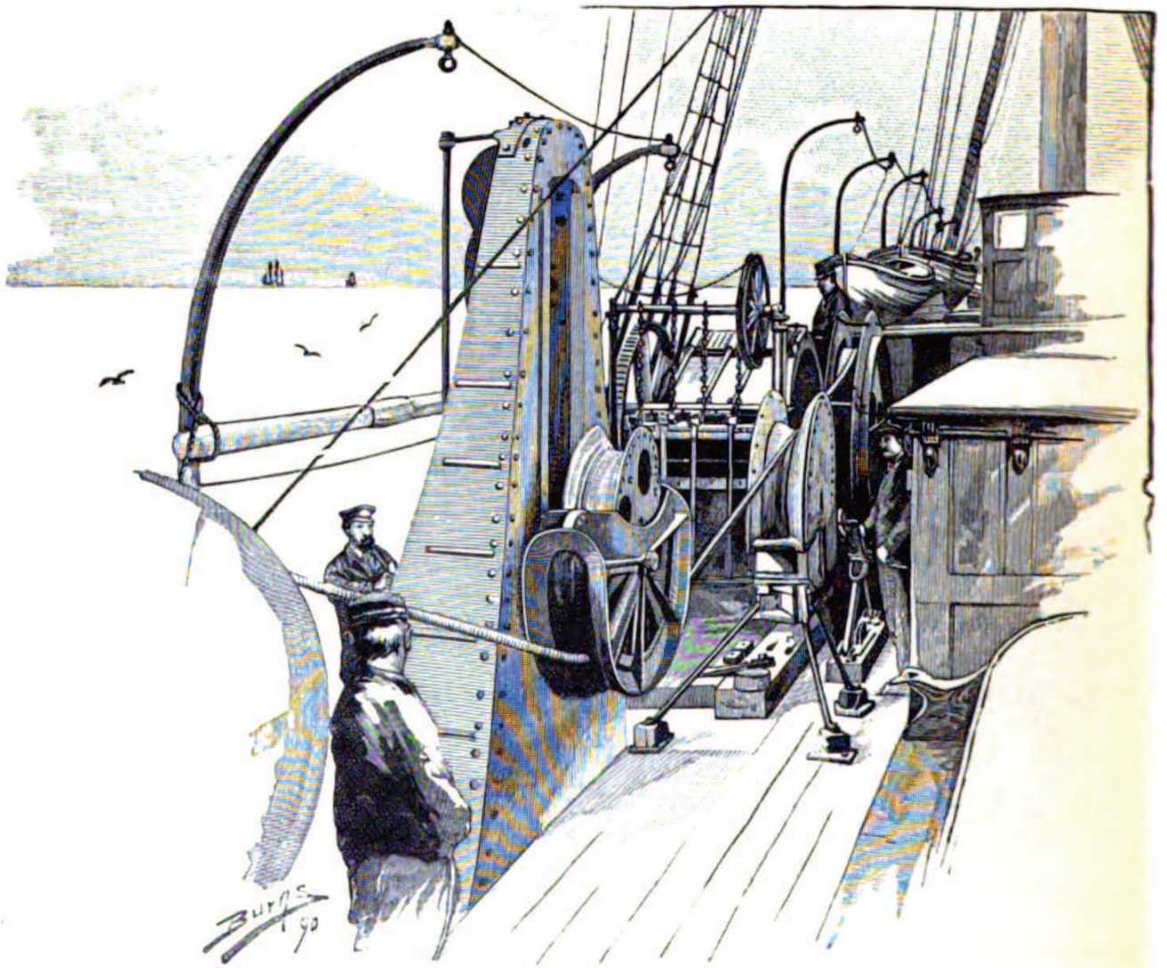
Paying-out Gear. From Stern Baulks.
