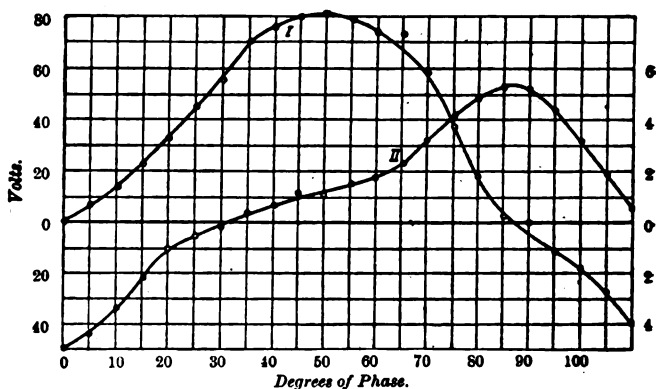
FIG. 204.—Primary Current Curve II and Primary Electromotive Force Curve I of the same Transformer taken off Wechsler Alternator.
