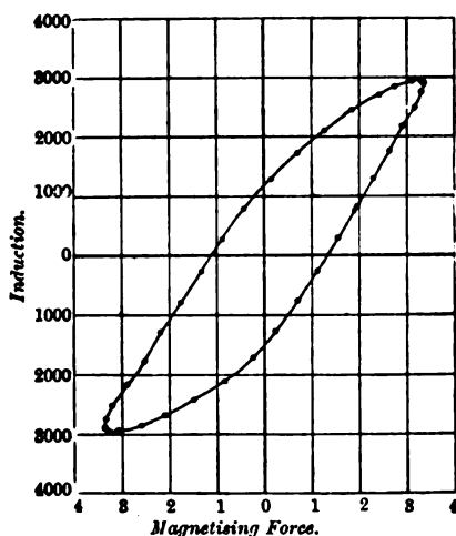
FIG. 195.—Hysteresis Curve of a Ganz Transformer.
