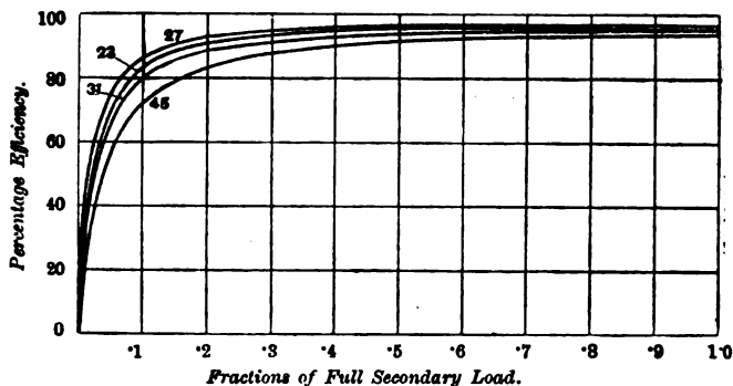
FIG. 197.—Efficiency Curves of Transformers.
