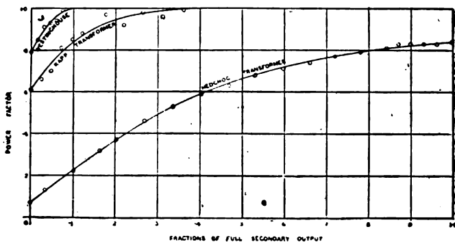
FIG. 201.—Relation of Power Factor to Secondary Output.
