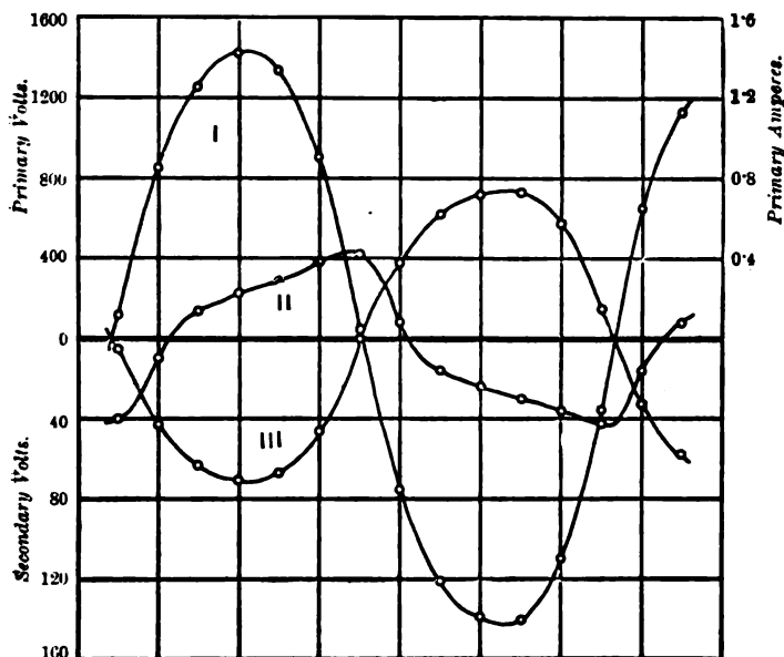
FIG. 186.—Primary E.M.F. Curve (I), Primary Current Curve (II) and Secondary E.M.F. Curve (III) of 10-light Westinghouse Transformer on Open Secondary Circuit.
