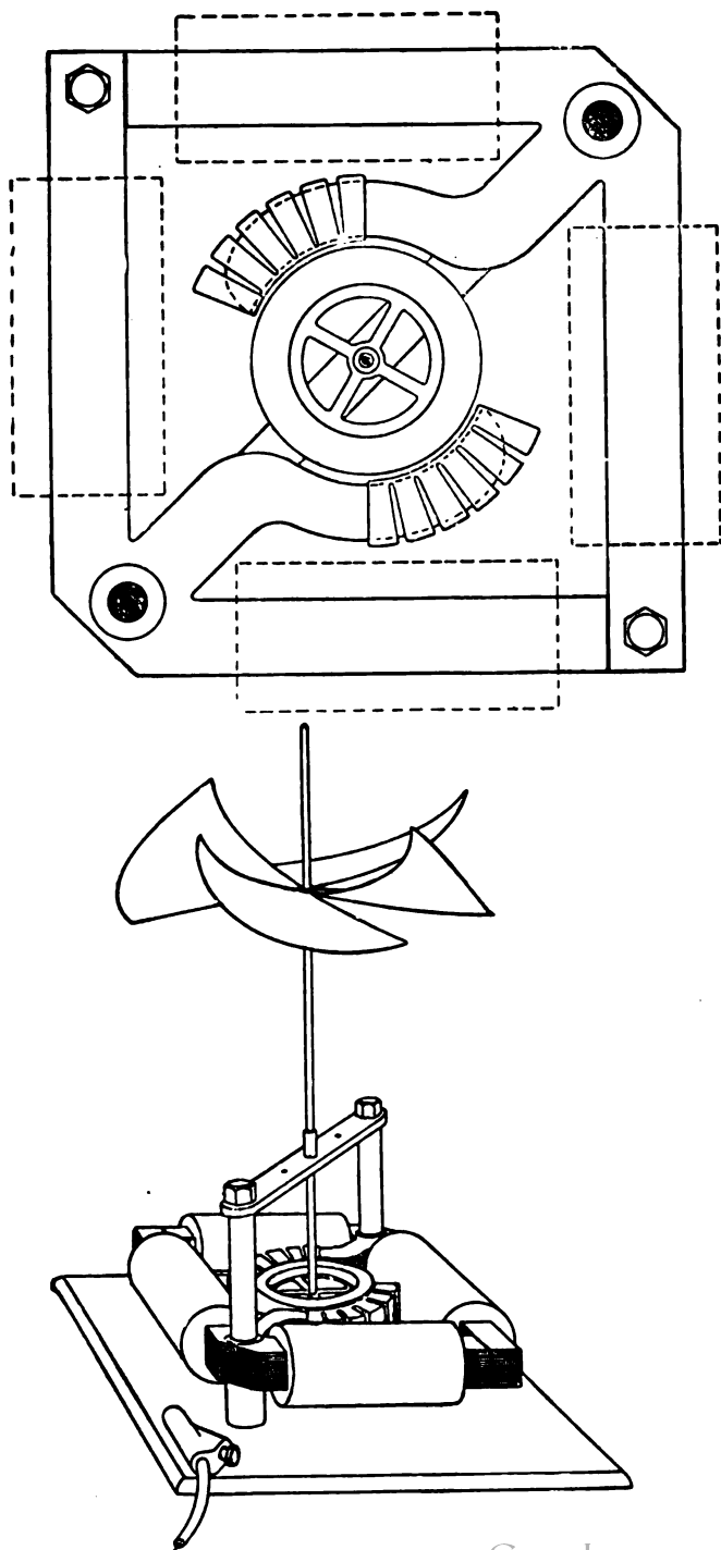
FIG. 126.—Plan and General View of Wright-Ferranti Self-starting Alternating Motor working a Fan.
