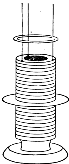
FIG. 116.—Aluminium Ring projected from the pole of an Alternating Electro-magnet, and floating over the pole when restrained by three strings.
