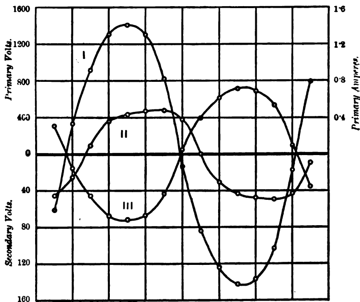
FIG. 187.—Primary E.M.F. Curve (I), Primary Current Curve (II) and Secondary E.M.F. Curve (III) of 10-light Westinghouse Transformer, loaded to one-tenth of full load.
