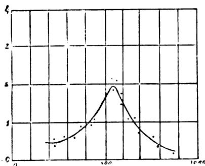
FIG. 155.—Curve showing relation between length of side of rectangle (taken as abscissa) and maximum sparking distance (taken as ordinate), the sides consisting of spirals gradually drawn out.
