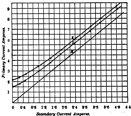
FIG. 205.—Current Diagram of a certain Transformer. Curve I, Primary Current taken with Ganz Alternator. Curve II, Primary Current taken with Wechsler Alternator. Curve III, twice value of Secondary Current. Transformation ratio of Transformer = 2:1.
