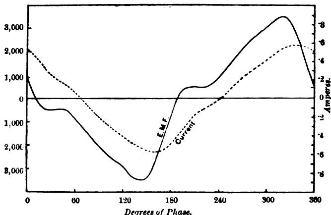
FIG. 181.—Primary E.M.F. and Primary Current Curves of Mordey Transformer, on Open Secondary Circuit, supplied off Thomson-Houston Alternator, furnishing Current also to other Transformers lightly loaded.
