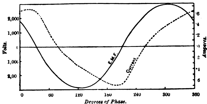
FIG. 178.—Primary E.M.F. and Primary Current Curves of Thomson-Houston Transformer, on Open Secondary Circuit, supplied off Mordey Alternator, with no other load.
