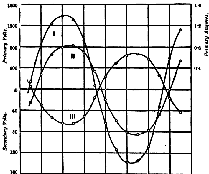
FIG. 189.—Primary E.M.F. Curve (I), Primary Current Curve (II) and Secondary E.M.F. Curve (III) of 10-light Westinghouse Transformer at full load.
