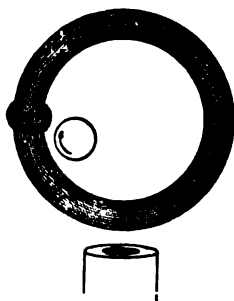
FIG. 127. —Magnetic Leakage across a Throttled Iron Ring, causing rotation of an Iron Disc placed near the Secondary Coil.
