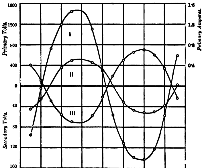
FIG. 188.—Primary E.M.F. Curve (I), Primary Current Curve (II) and Secondary E.M.F. Curve (III) of 10-light Westinghouse Transformer loaded to half load.
