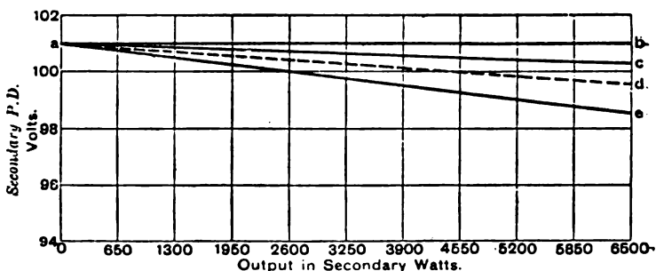
FIG. 202.—Secondary Drop Curves of 6,500-watt Westinghouse Transformer.
