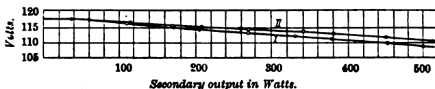
FIG. 209.—Curve of Secondary Drop of Transformer. Curve I taken on Ganz Alternator. Curve II taken on Wechsler Alternator.
