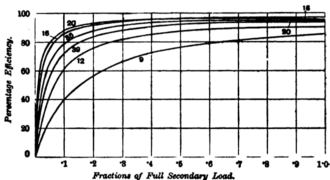
FIG. 196.—Efficiency Curves of Transformers.
