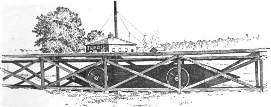
Fig. 13.—The Weems System for a High-speed Electric Railway. More than one hundred and twenty miles an hour actually accomplished on an experimental Track.
