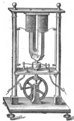
Fig. 1.—Pixii's Magneto-electric Machine, 1832.
