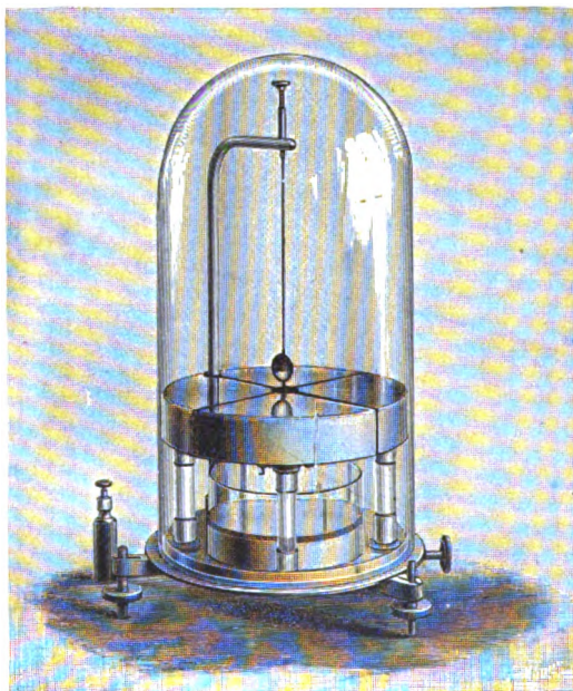
Thomson's Quadrant Electrometer, for comparing potentials.
