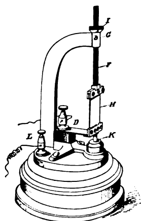
Fig. 17.—Maxim's Incandescent Platinum Lamp.
