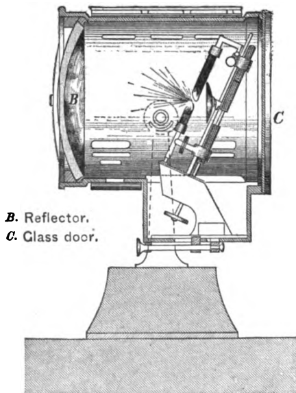
Sectional View of Ship's Search-light.
