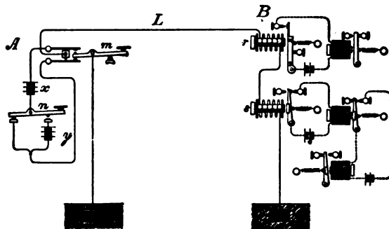
The Duplex System, for simultaneously sending two messages in the same direction on a single wire.
