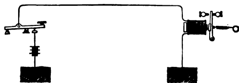
The Modern Morse Telegraph.
