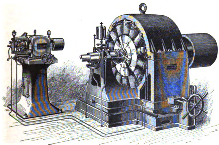
Fig. 24.—An Alternating Current Dynamo and Exciter.
