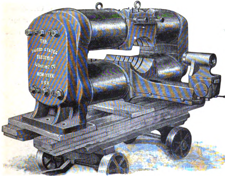
Fig. 9.—Field Magnets and Frame, without armature.
