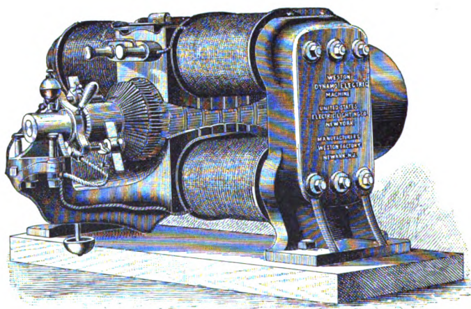
Fig. 10.—A Complete Dynamo—armature in place.
