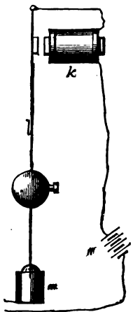
FIG. 34. PENDULUM CIRCUIT BREAKER.
