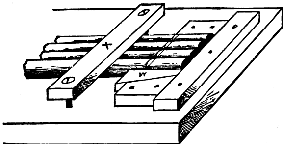
FIG. 1.—MAKING NEGATIVE PLATES FROM ARC LIGHT CARBONS.
