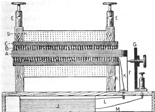
FIG. 37. INDUCTION COIL.
