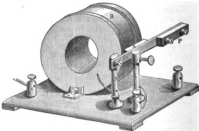
FIG. 41. RECORDON'S INDUCTION COIL.
