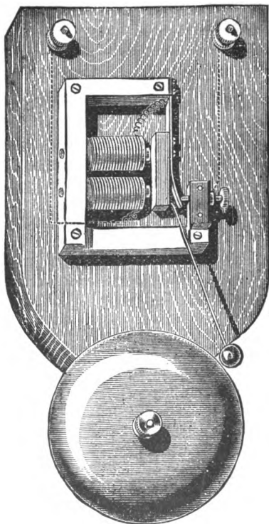
FIG. 26. THE VIBRATING BELL.
