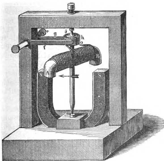
FIG. 21. PAGE'S ROTATING ARMATURE.
