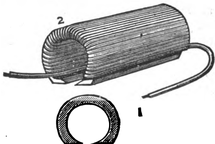
FIG. 13. JOULE'S ELECTRO-MAGNET.
