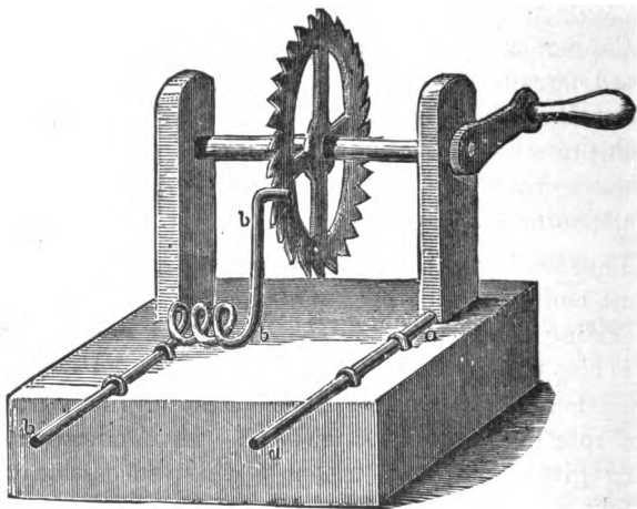
FIG. 46. CIRCUIT BREAKER.
