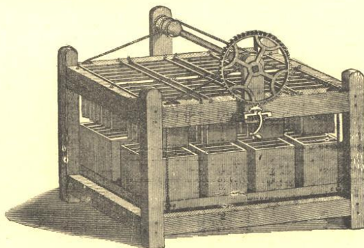
FIG. 1.—Galvanic Battery.
