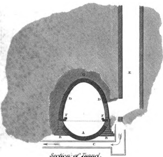
Section of Tunnel.
