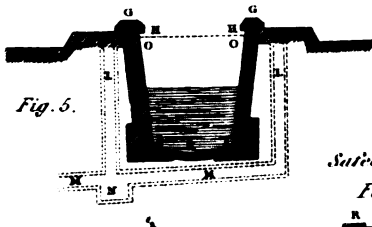
Section of a Lock.
