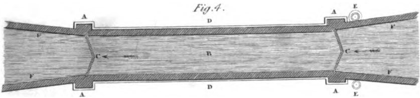
Plan of a Lock.
