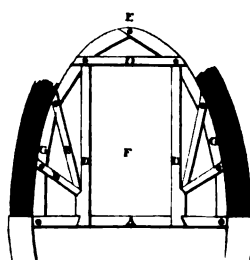
Centering to Soffit Arch.
