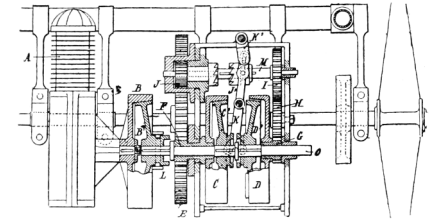
Cherrier Two-Speed Gear, 1900
