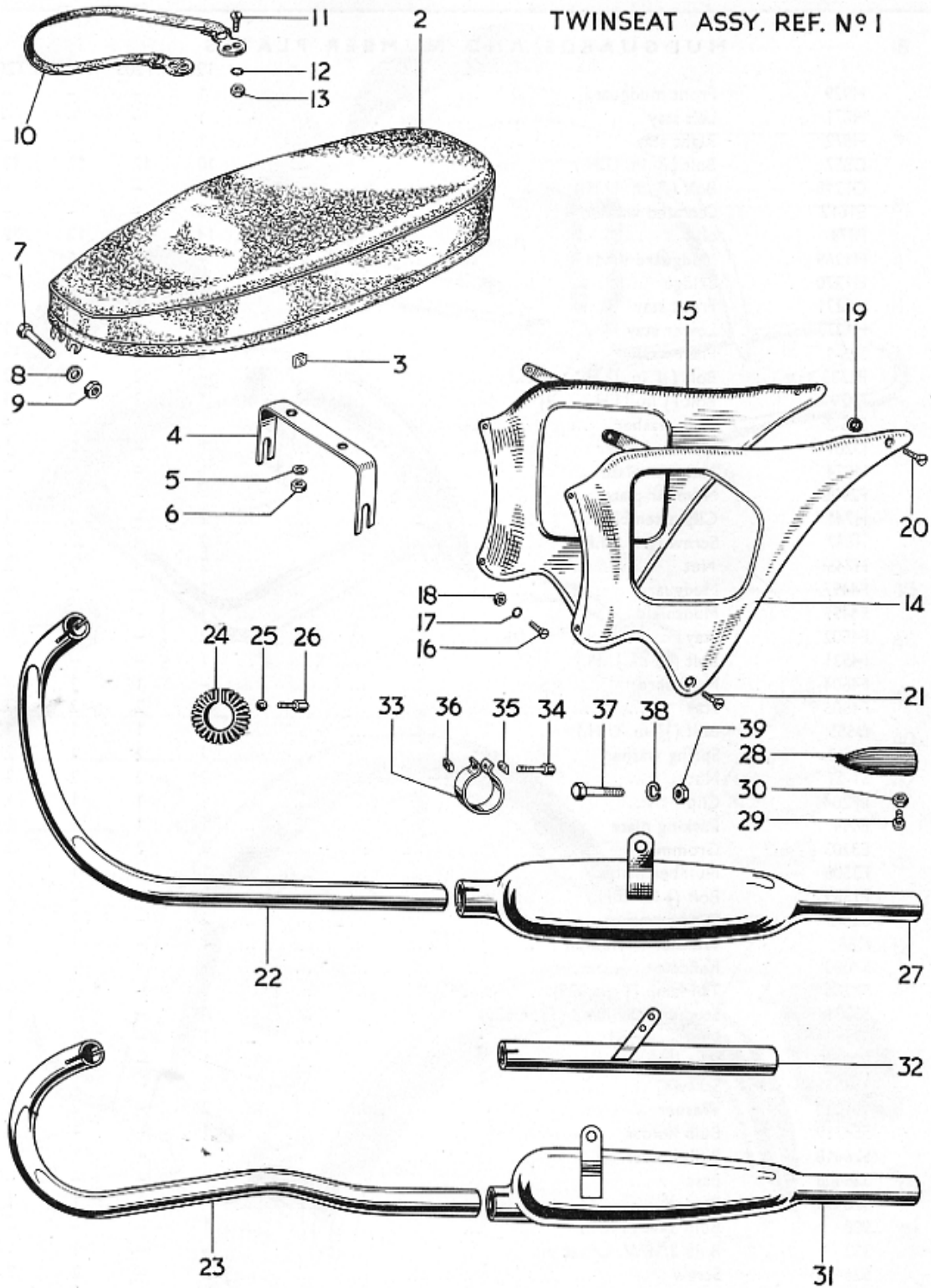
Fig. 20. TWINSEAT, REAR PANELS AND EXHAUST SYSTEM.
