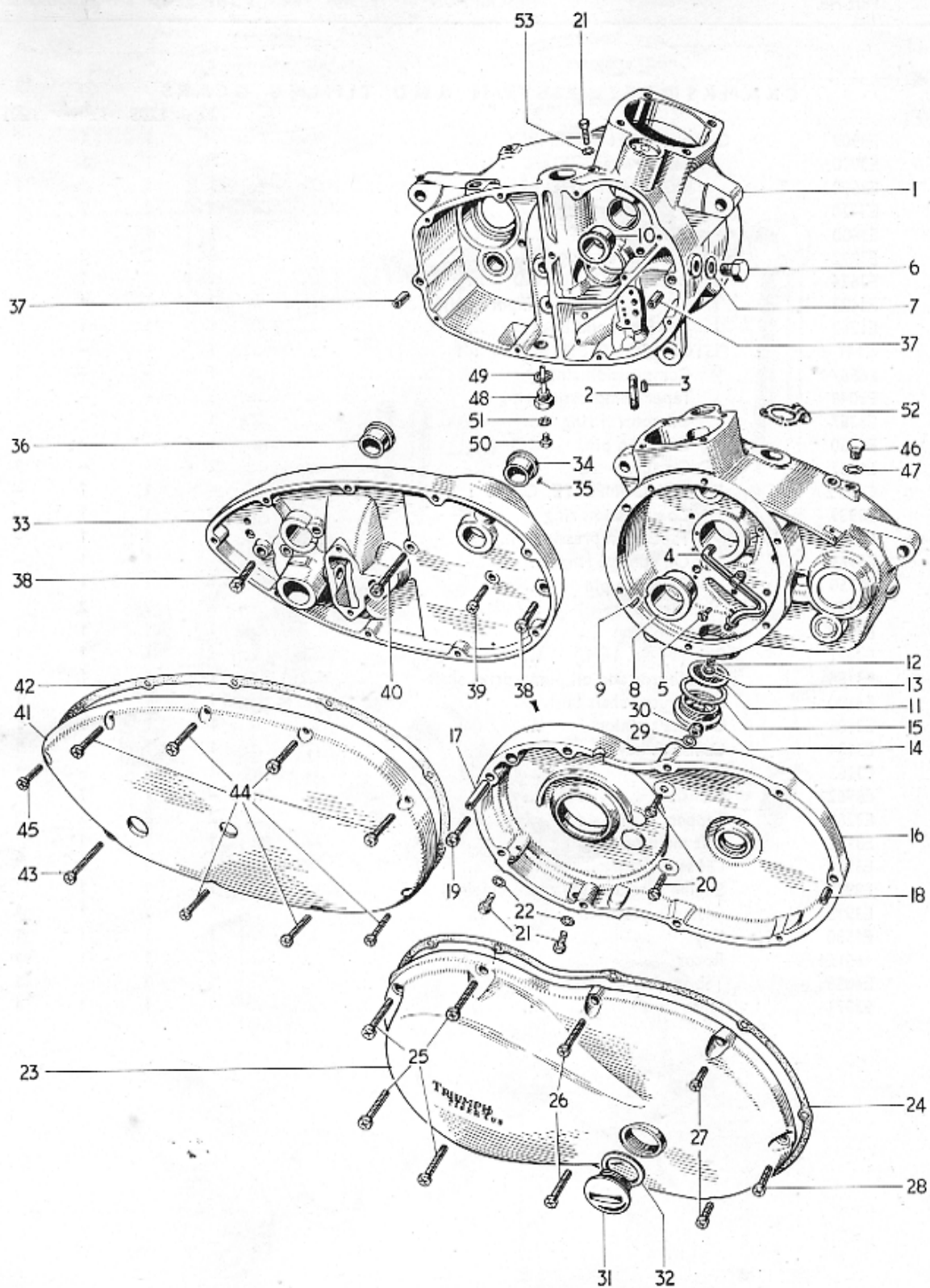
Fig. 2. CRANKCASE (ONE-PIECE) UP TO ENGINE No. 57616
