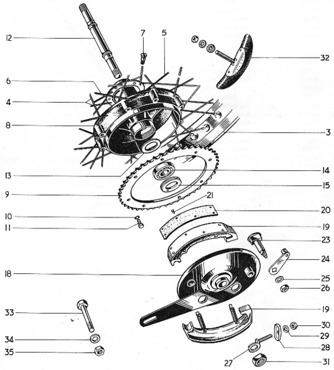
Fig. 16. REAR WHEEL.
