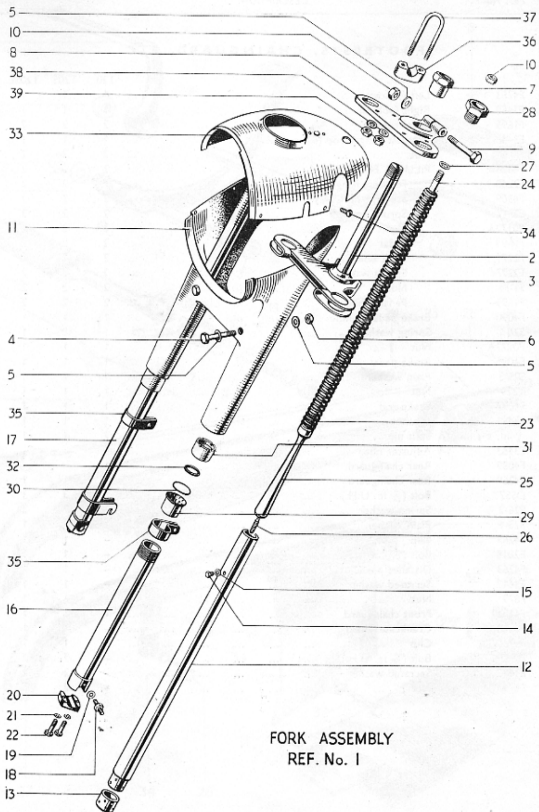
Fig. 10. TELESCOPIC FRONT FORK T20
