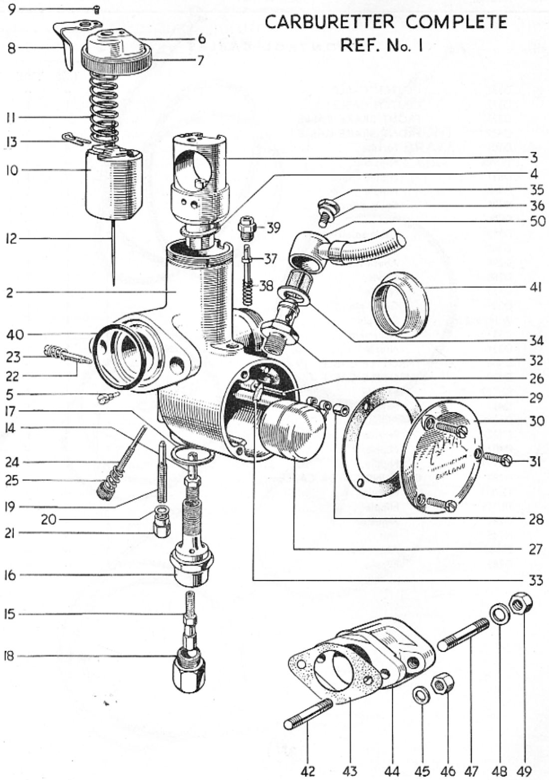
Fig. 23. AMAL CARBURETTER.
