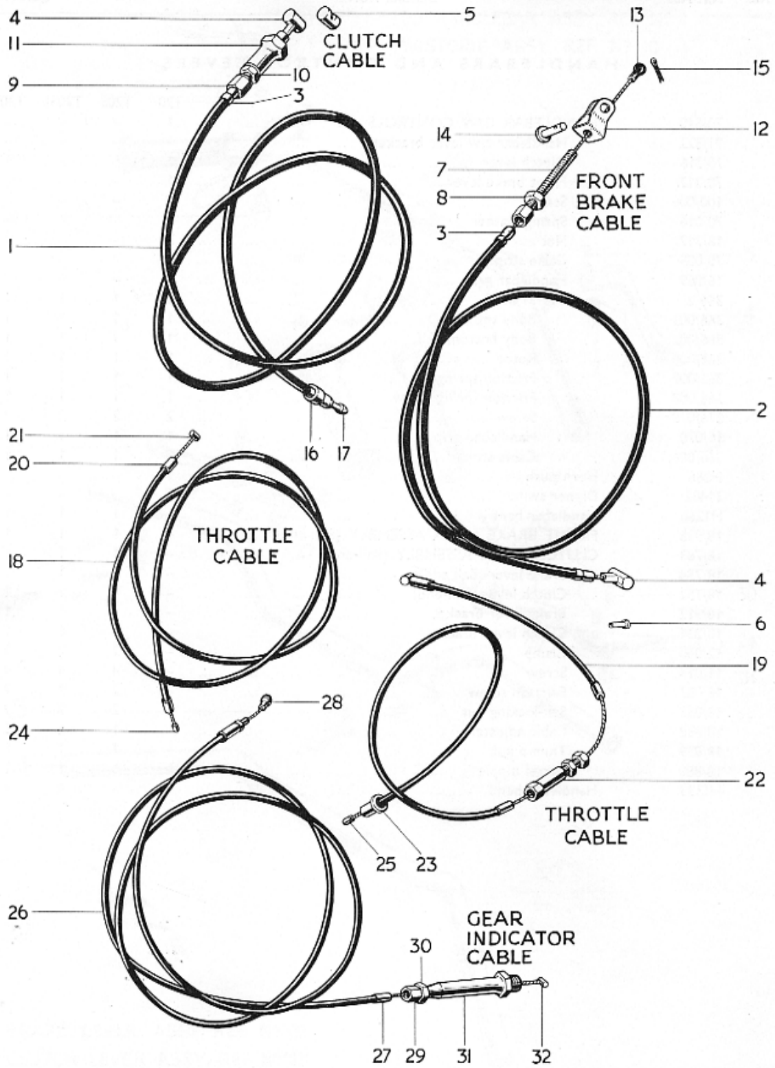
Fig. 22. CONTROL CABLES.
