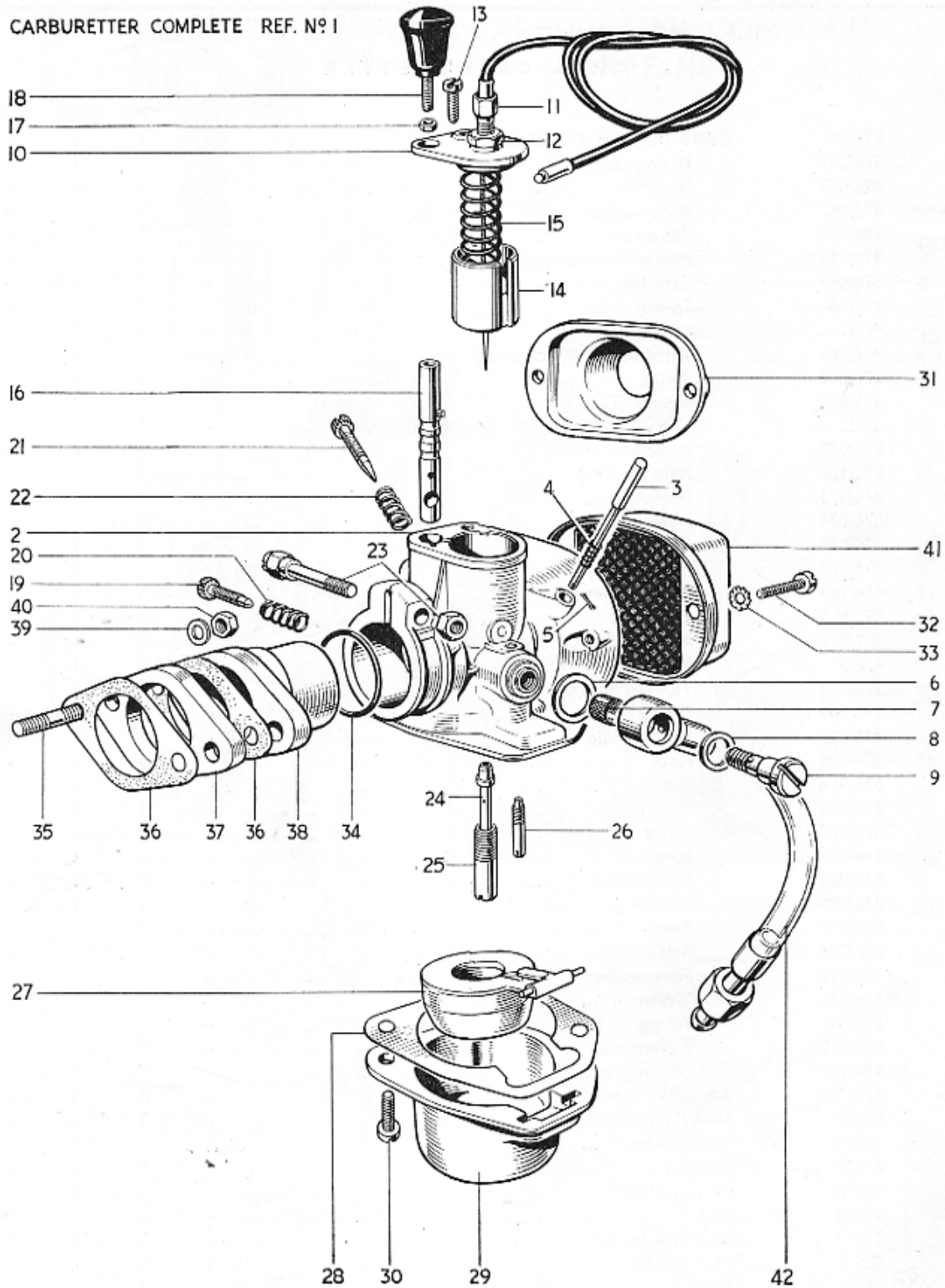
Fig. 24. ZENITH CARBURETTER.
