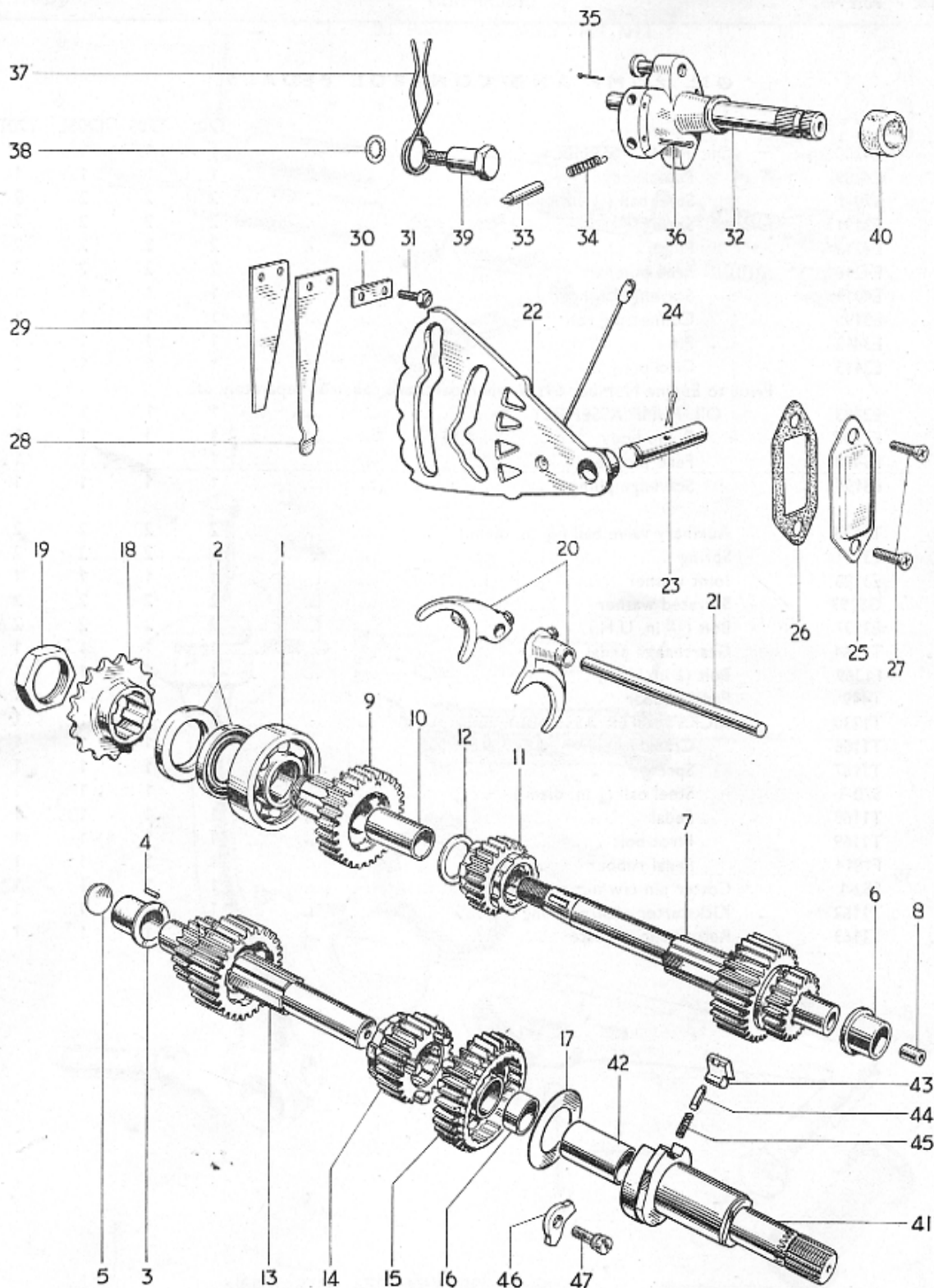
Fig. 6. GEARBOX SHAFTS AND GEARS
