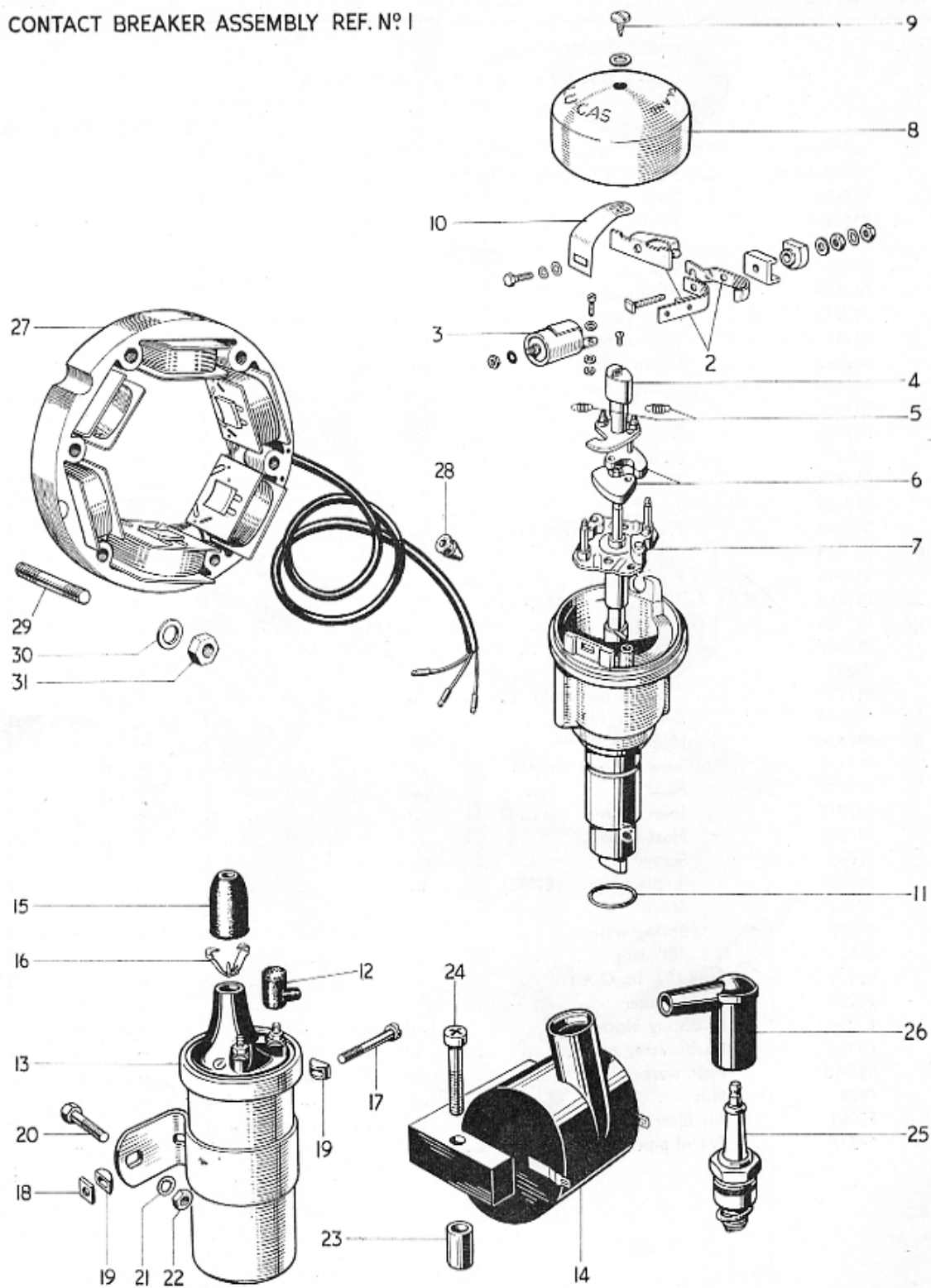
Fig. 25. CONTACT BREAKER, COIL AND STATOR.
