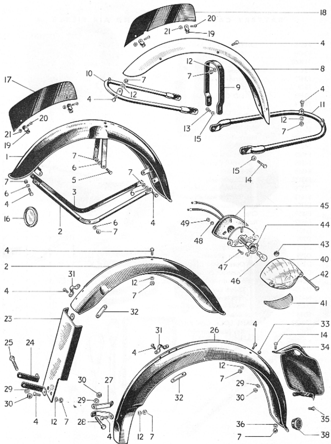
Fig. 19. MUDGUARDS AND NUMBER PLATES.
