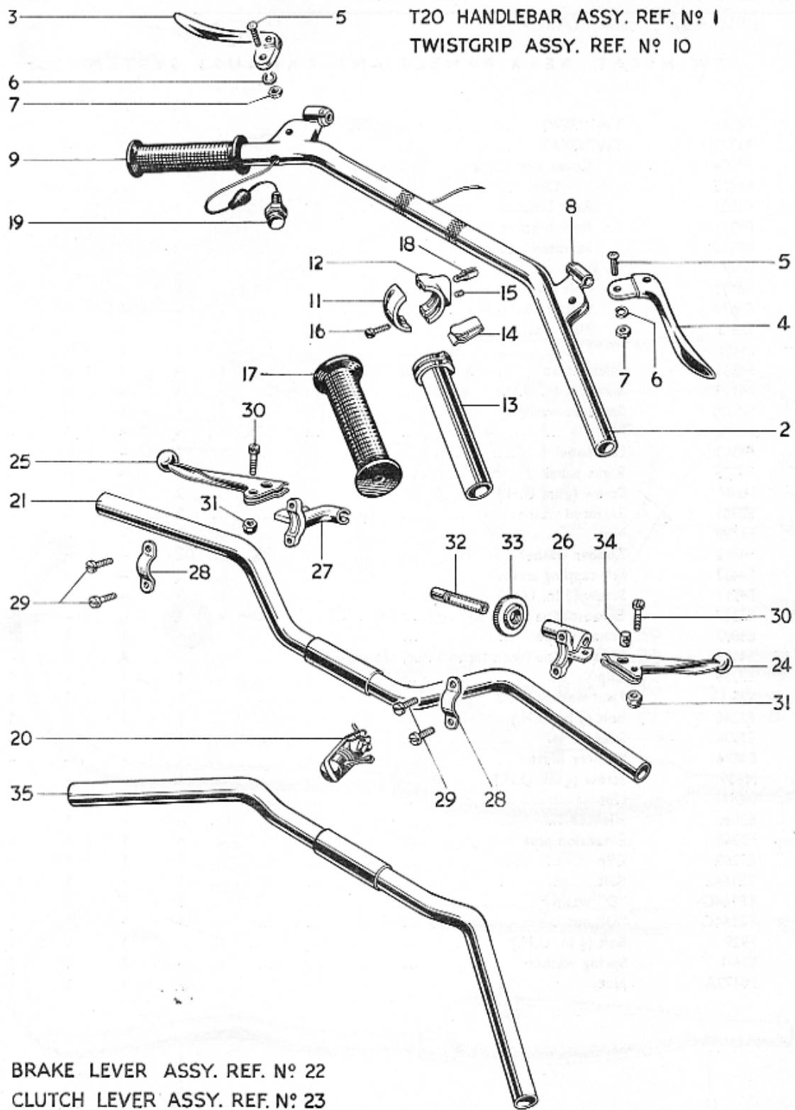
Fig. 21. HANDLEBARS AND CONTROL LEVERS.
