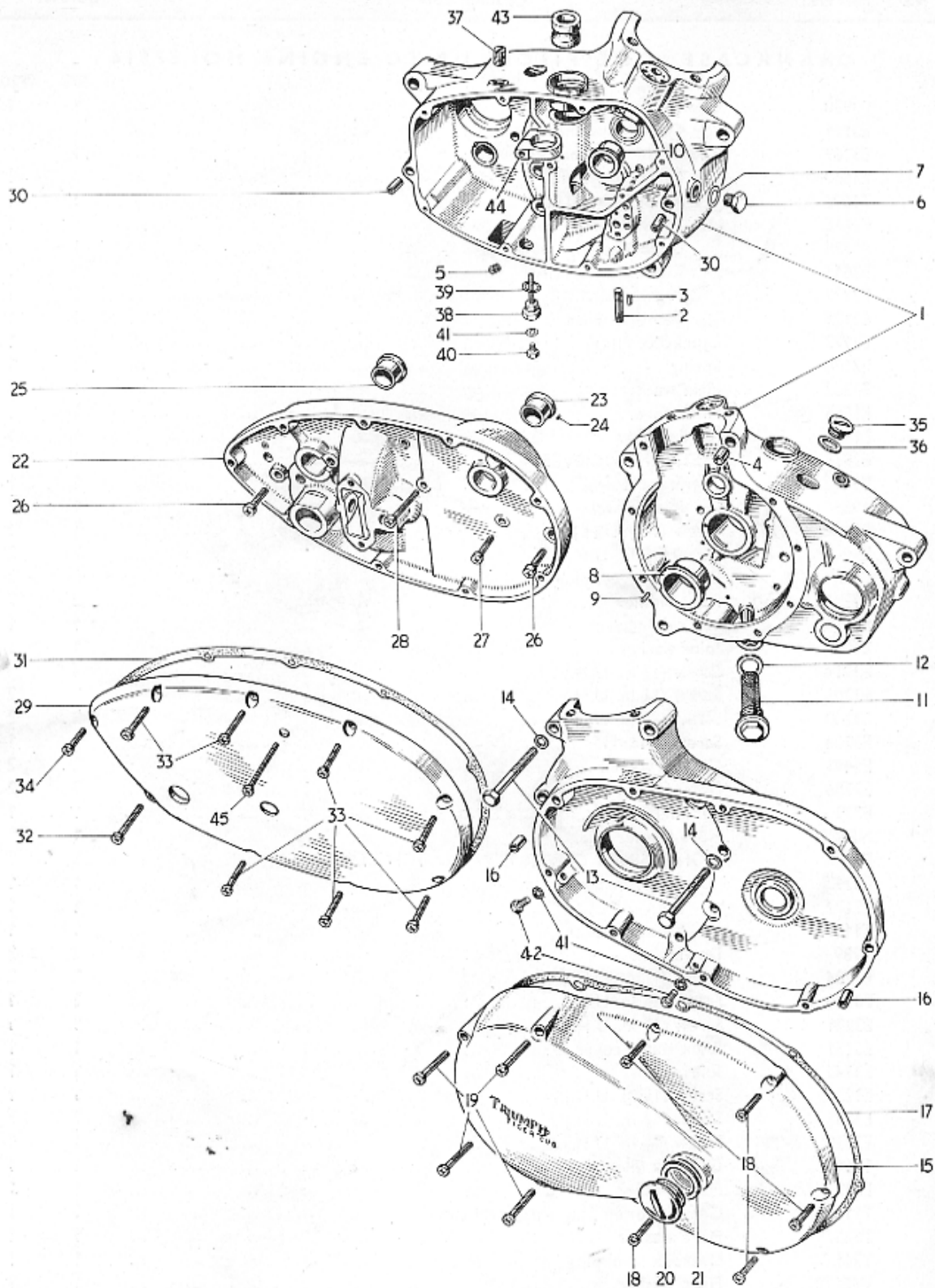
Fig. 3. CRANKCASE (TWO-PIECE) FROM ENGINE No. 57617
