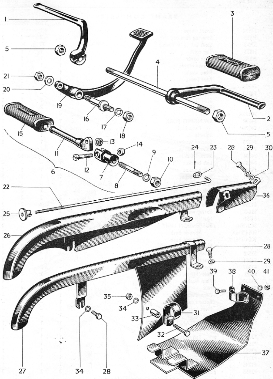
Fig. 9. FOOTRESTS, CHAINGUARD, Etc.
