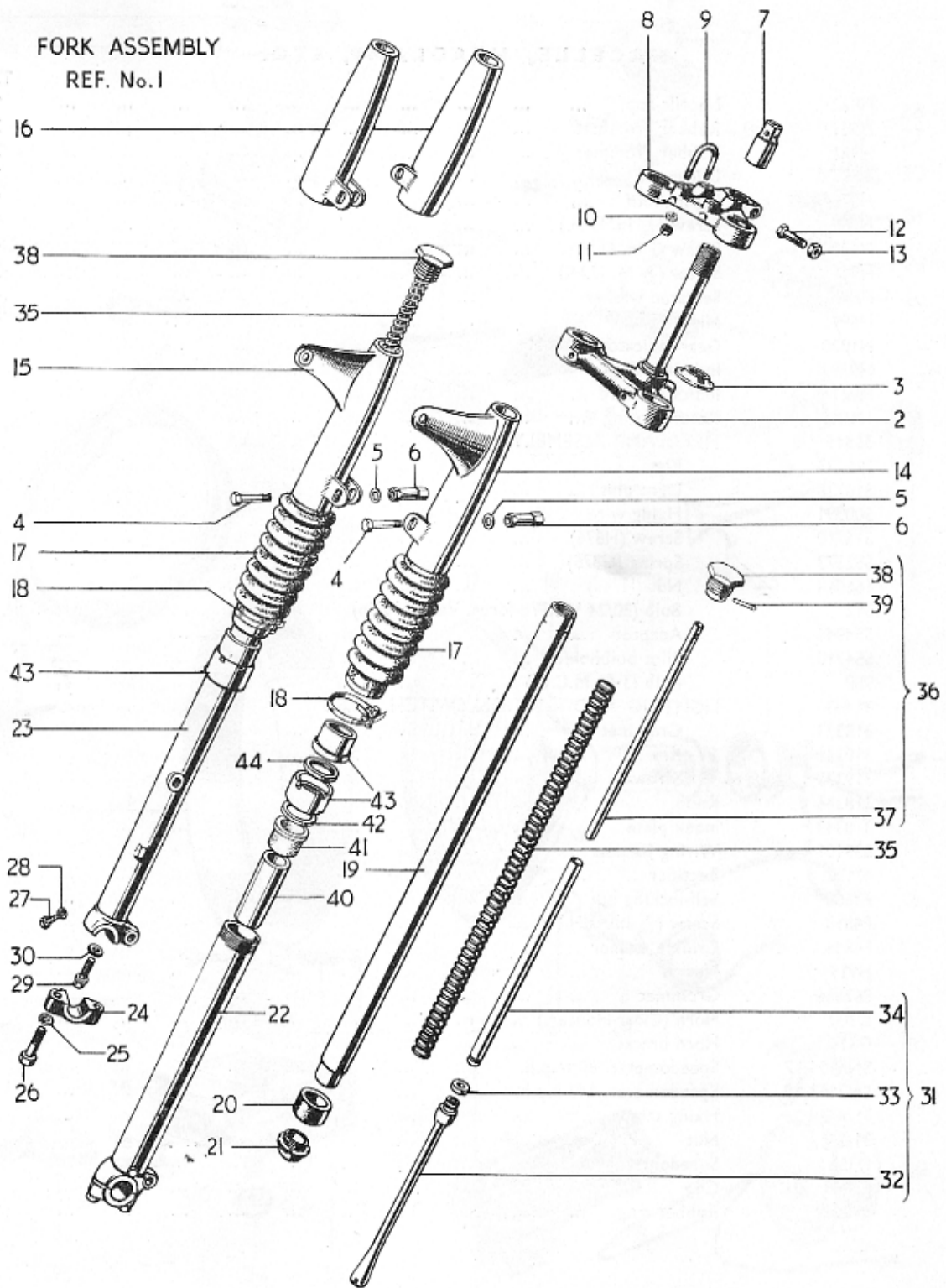
Fig. 12. TELESCOPIC FRONT FORK T20S, T20SL and T20T
