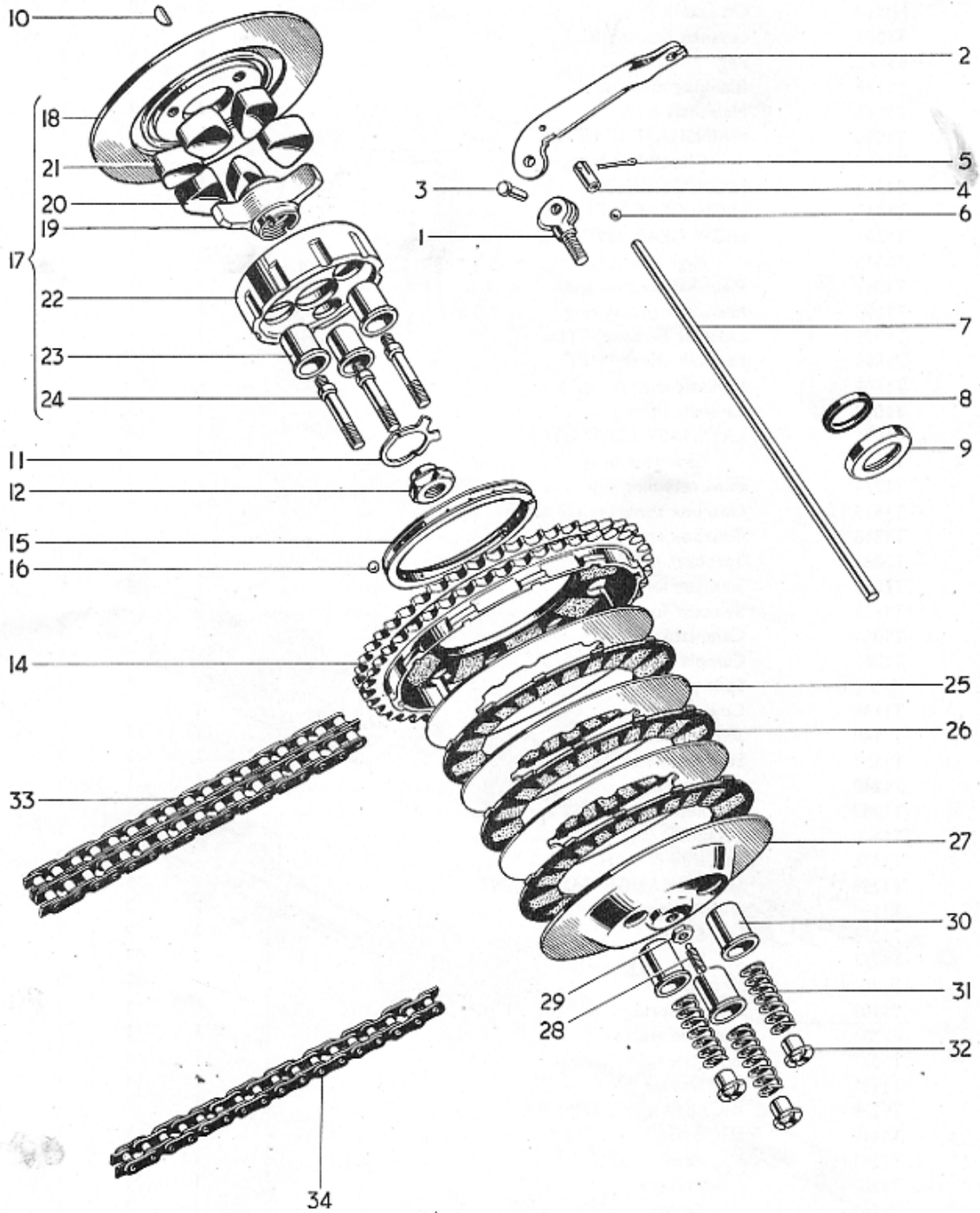
Fig. 7. CLUTCH AND CHAINS
