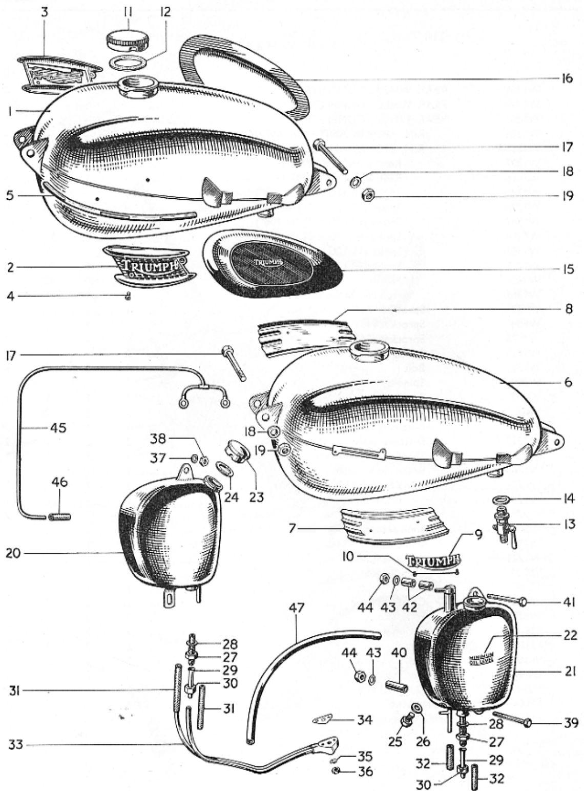
Fig. 17. PETROL AND OIL TANKS.
