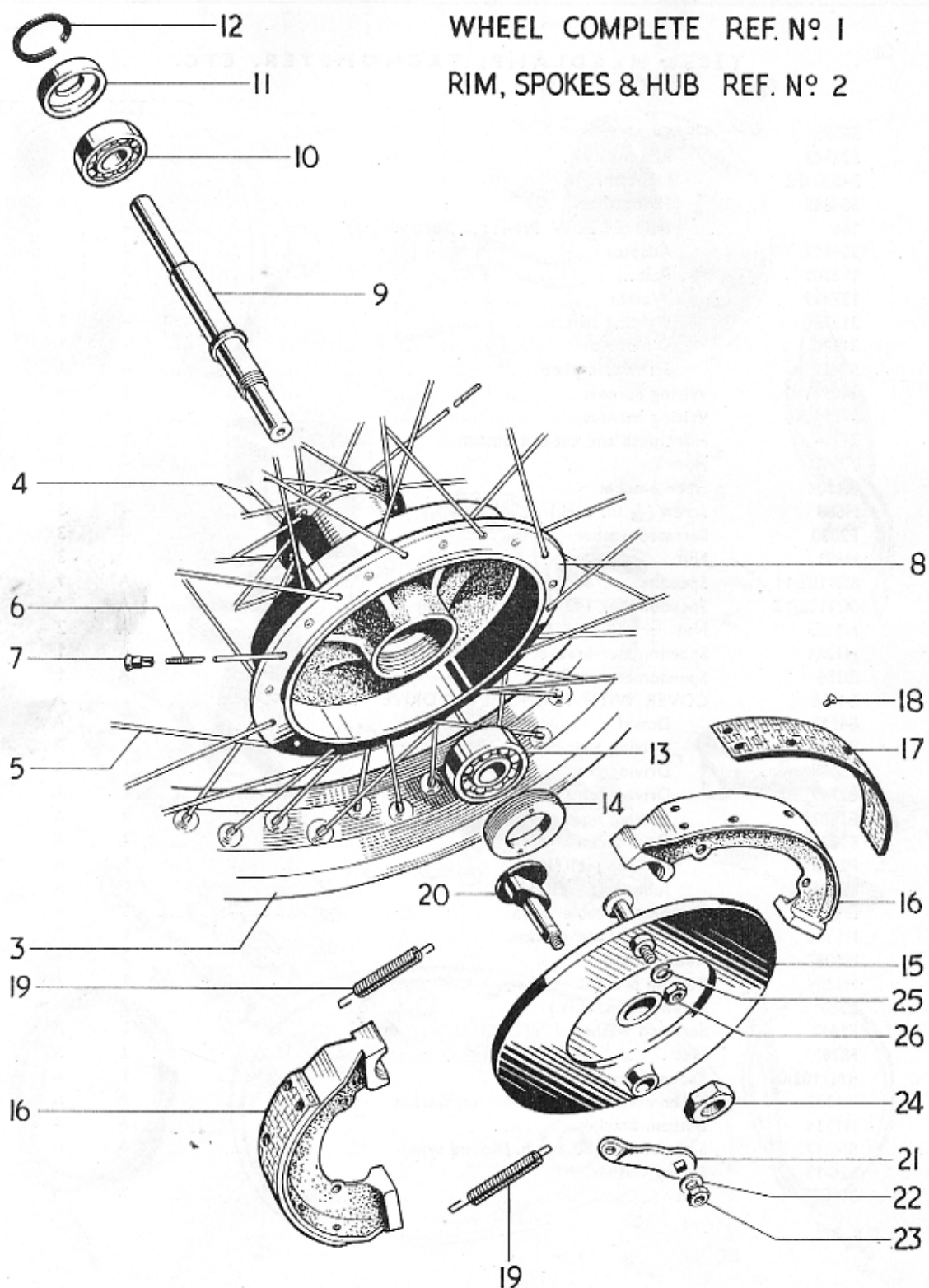
Fig. 14. FRONT WHEEL, T20.
