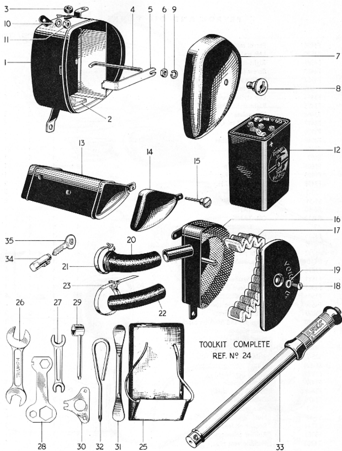
Fig. 18. BATTERY CASE, TOOLBOX AND AIR FILTER.
