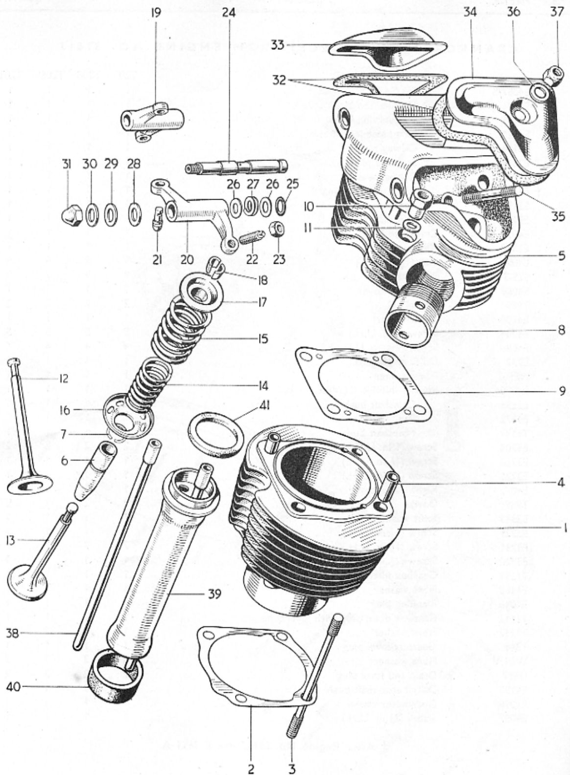
Fig. 4. CYLINDER BARREL AND HEAD
