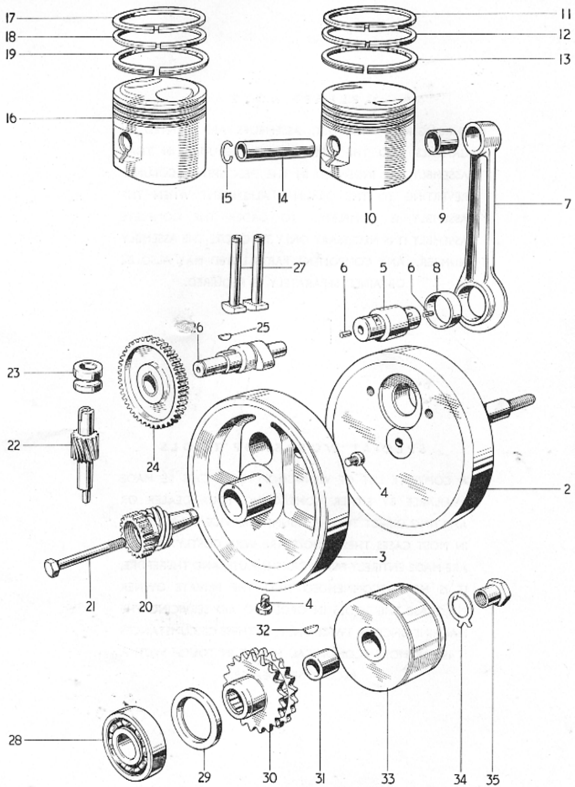
Fig. 1. CRANKSHAFT, PISTON AND TIMING GEARS
