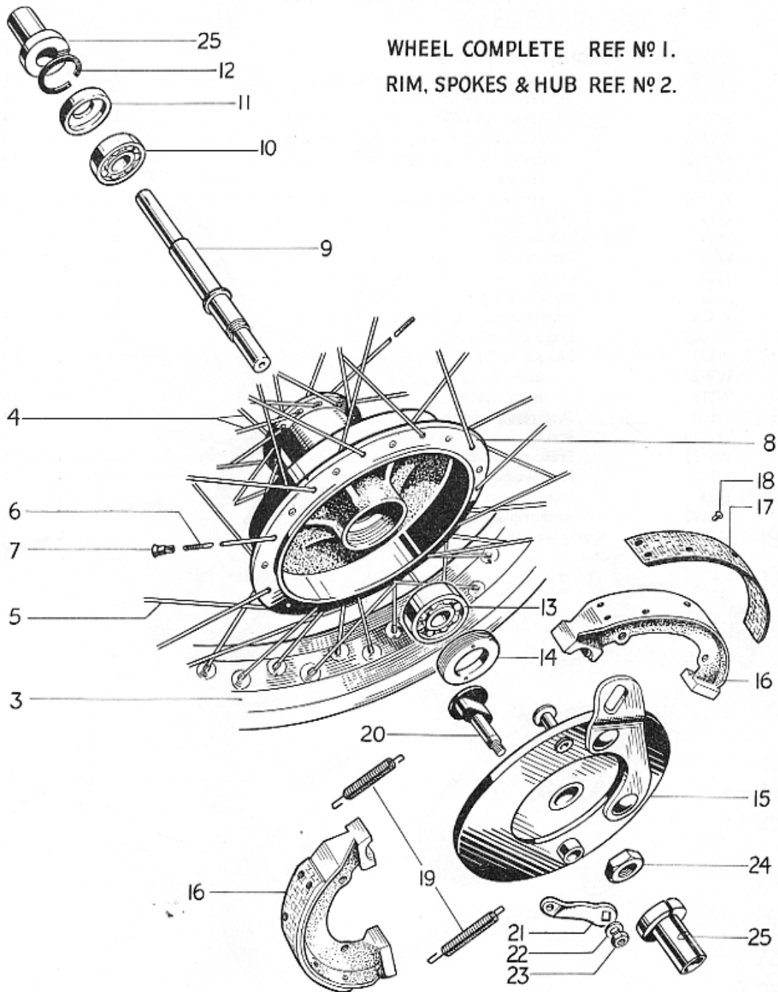
Fig. 15. FRONT WHEEL, T20S, T20SL & T20T.
