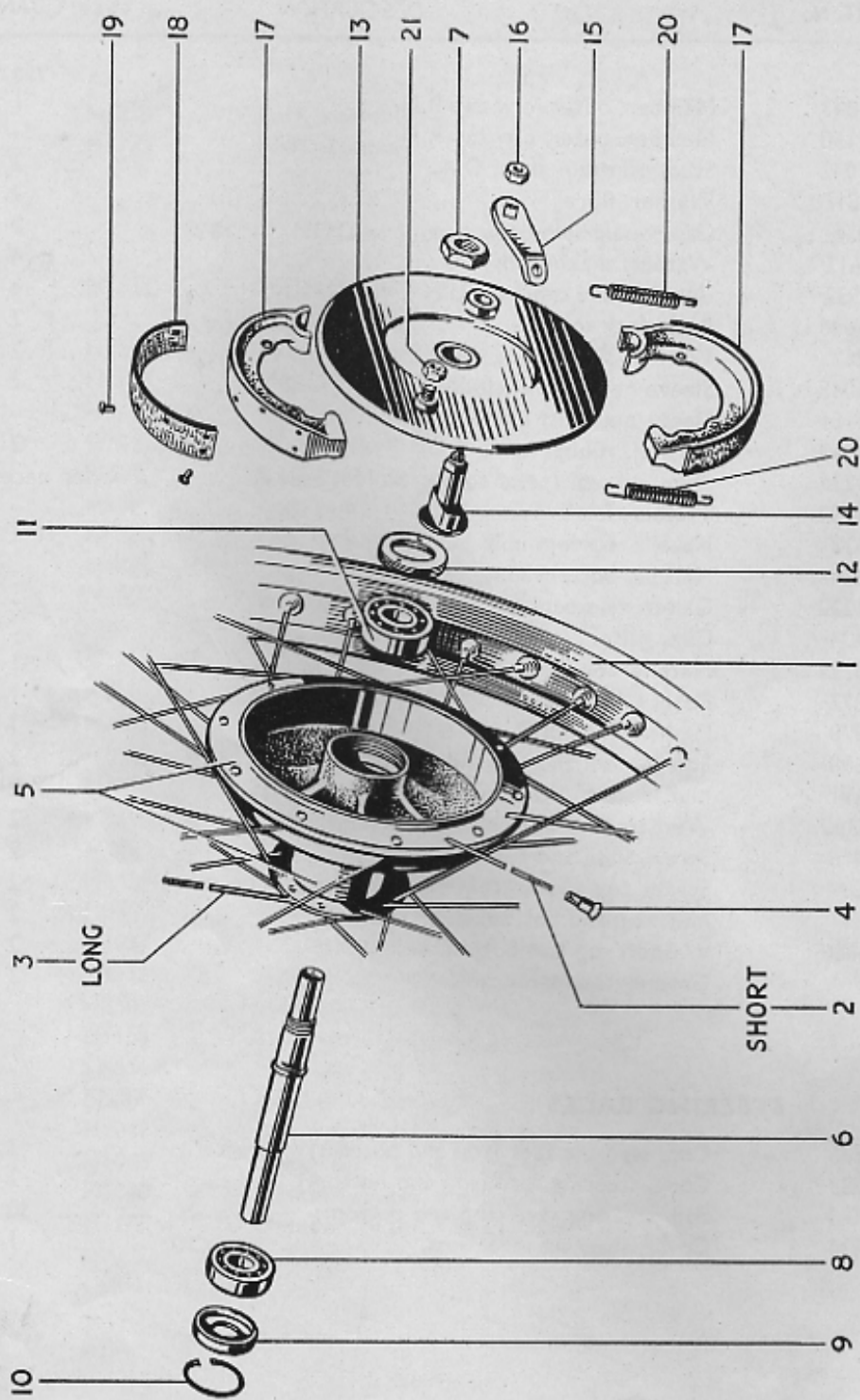
FIG. 7. FRONT WHEEL.
