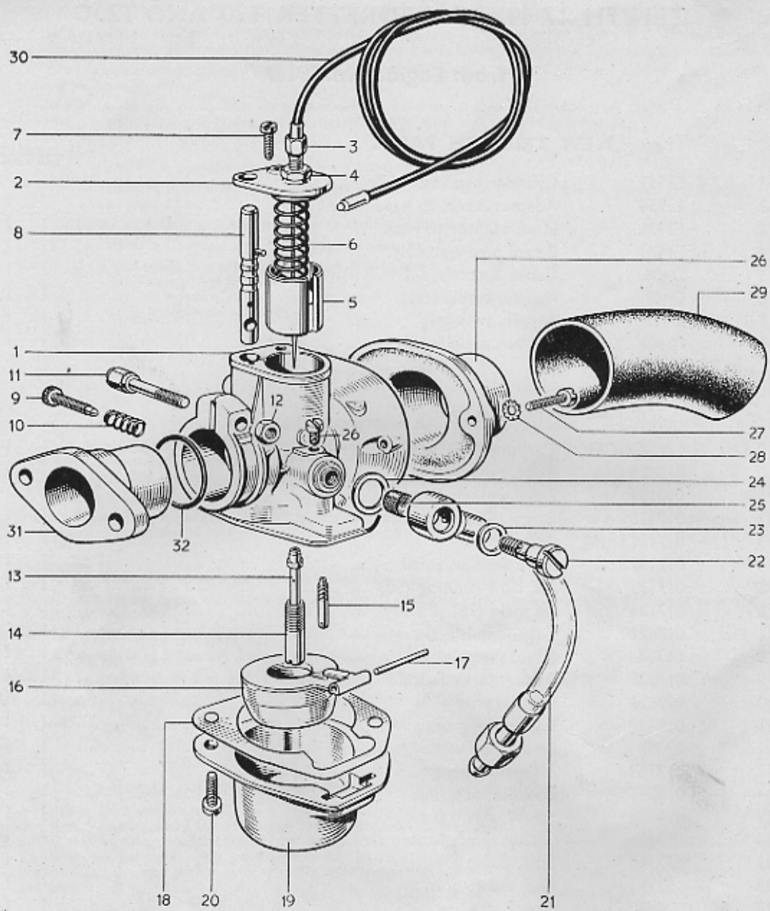
FIG. 15. ZENITH CARBURETTER
